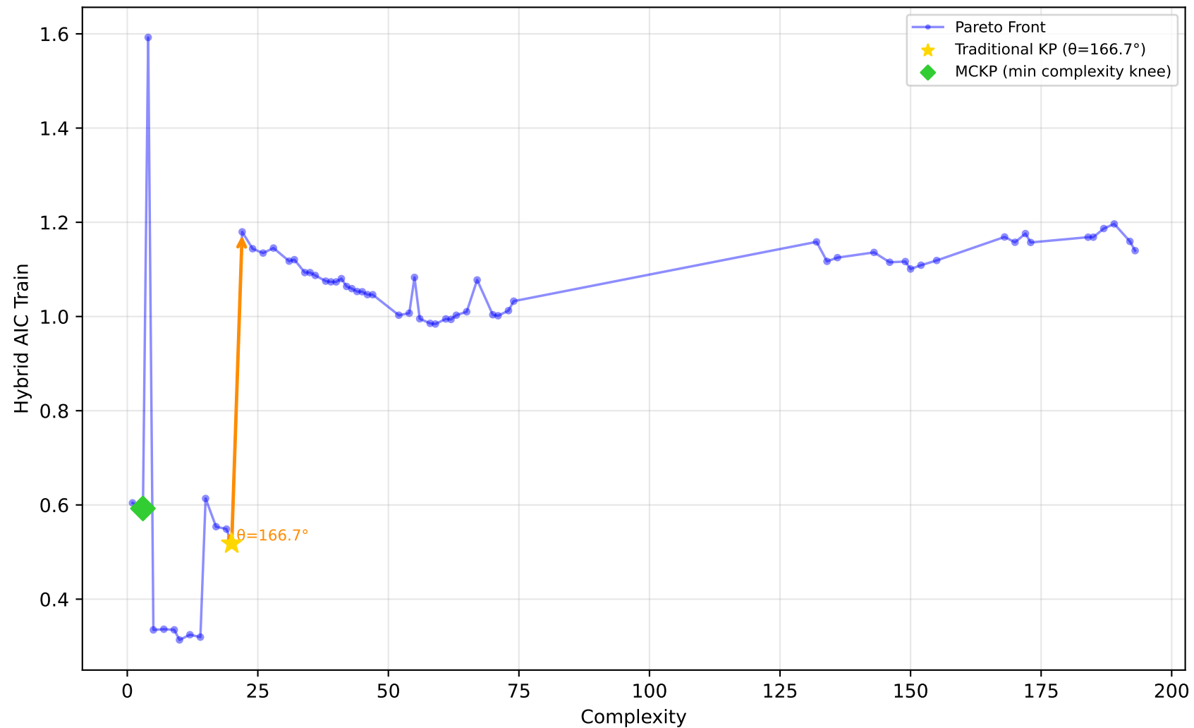
228_elusage - Run 20 - MVP - Hybrid AIC Train \lambda_1=0.00, \lambda_2=0.00, \lambda_3=1.00 | Difficulty: 1.00 | Method: hmr
