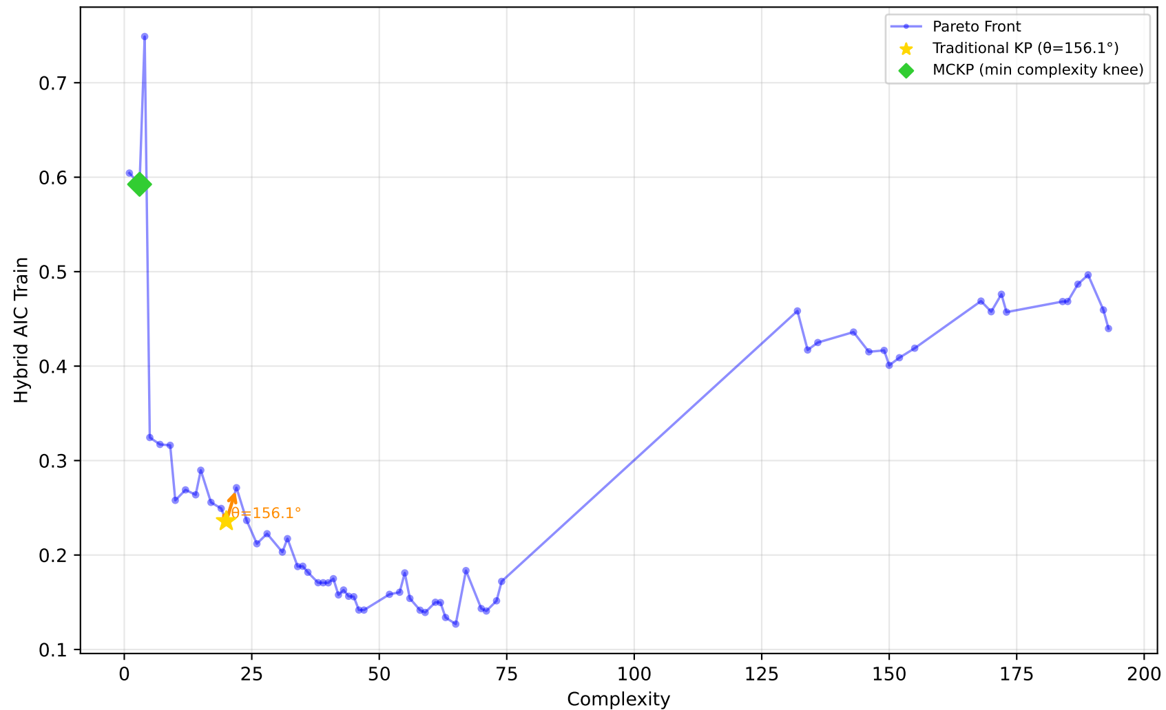
228_elusage - Run 20 - MVP - Hybrid AIC Train \lambda_1=0.00, \lambda_2=0.30, \lambda_3=0.00 | Difficulty: 1.00 | Method: hmr
