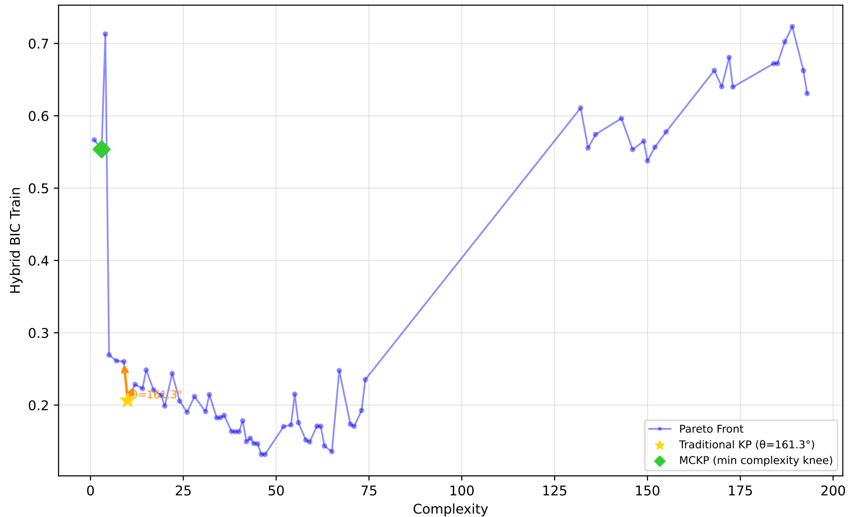
228_elusage - Run 20 - MVP - Hybrid BIC Train \lambda_1=0.00 , \lambda_2=0.30 , \lambda_3=0.00 | Difficulty: 1.00 | Method: hmr
