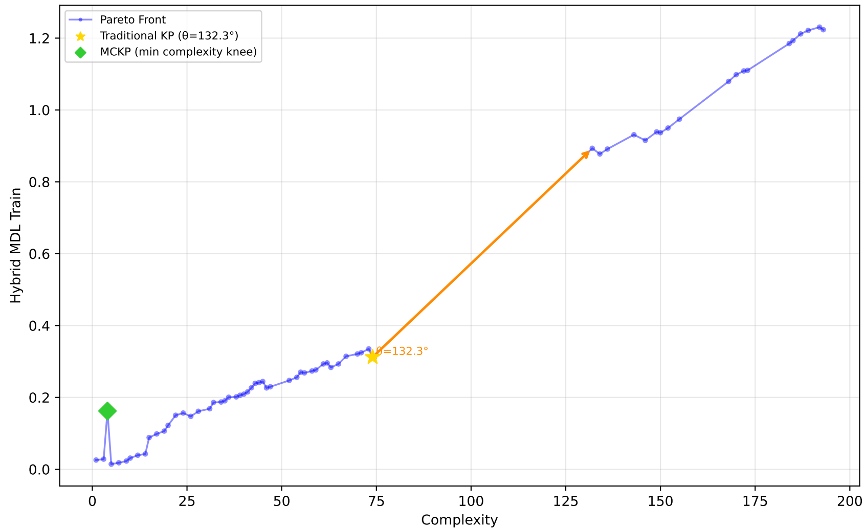
228_elusage - Run 20 - MVP - Hybrid MDL Train \lambda_1=0.00, \bar{\lambda}_2=0.30, \lambda_3=0.00 | Difficulty: 1.00 | Method: hmr
