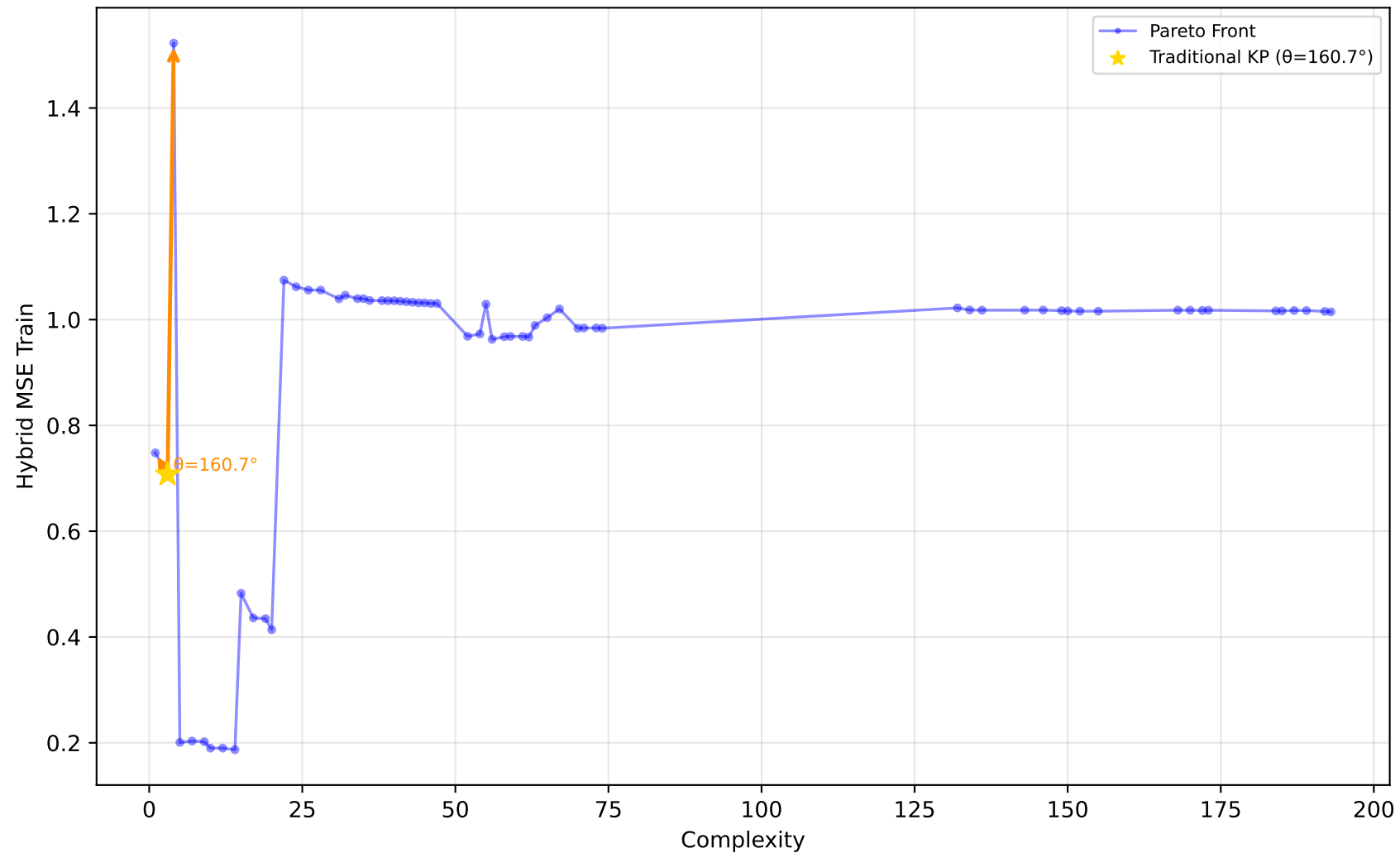
228_elusage - Run 20 - MVP - Hybrid MSE Train \lambda_1=0.00, \bar{\lambda}_2=0.00, \lambda_3=1.00 | Difficulty: 1.00 | Method: hmr
