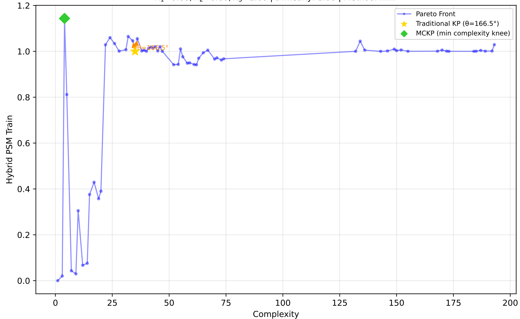
228_elusage - Run 20 - MVP - Hybrid PSM Train \lambda_1=0.00, \bar{\lambda}_2=0.00, \lambda_3=1.00 | Difficulty: 1.00 | Method: hmr
