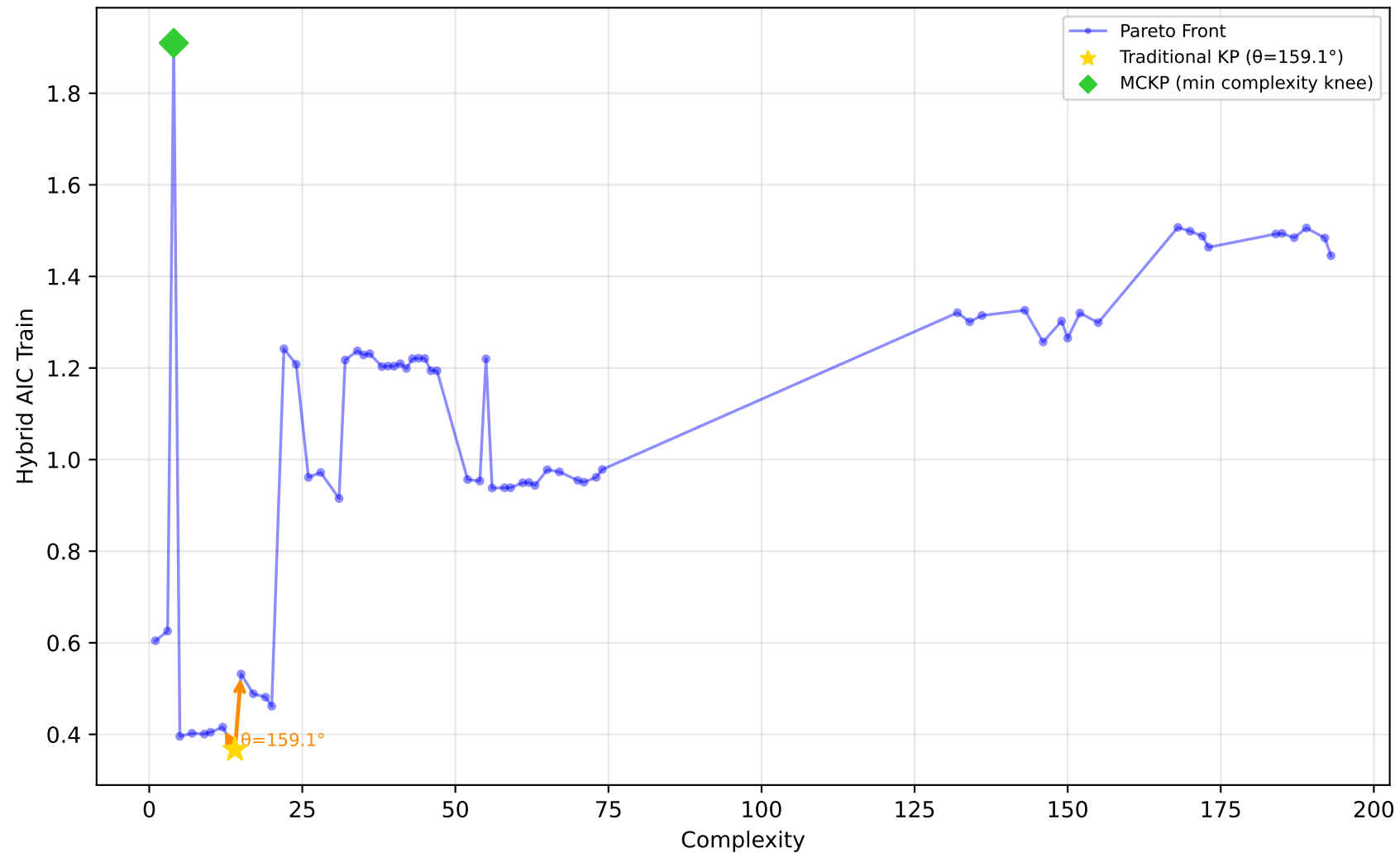
228_elusage - Run 20 - SVP - Hybrid AIC Train \lambda_1=0.60, \lambda_2=0.60, \lambda_3=1.00 | Difficulty: 1.00 | Method: hmr
