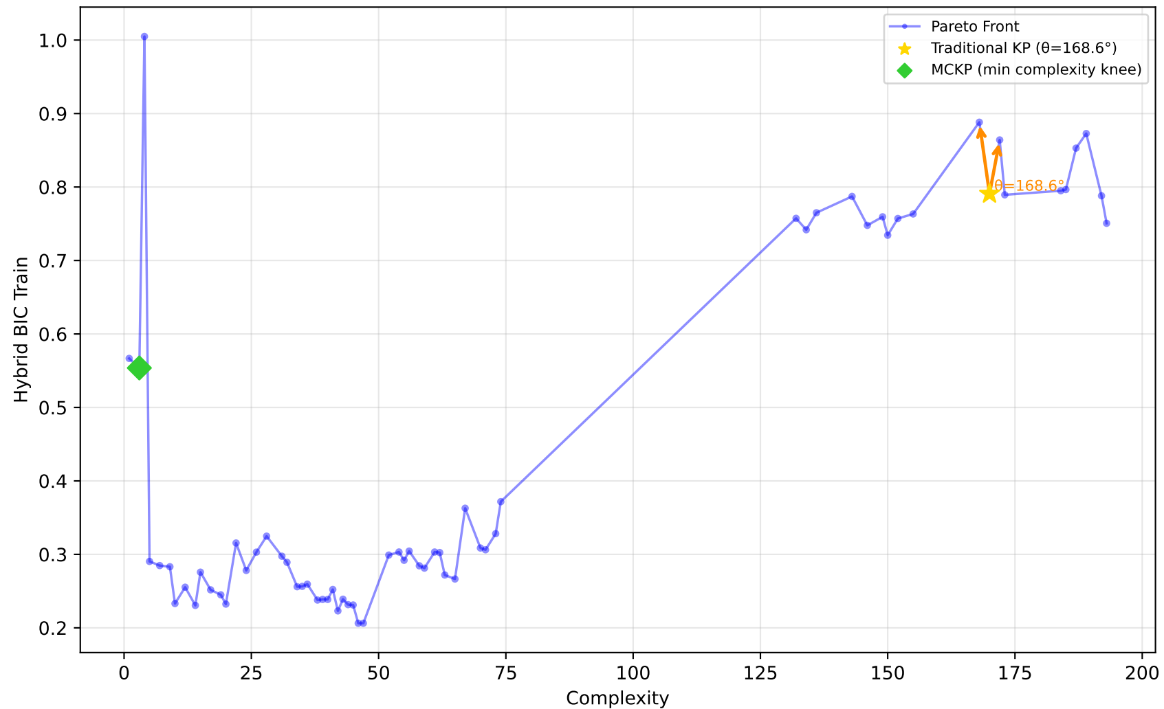
228_elusage - Run 20 - SVP - Hybrid BIC Train \lambda_1=0.00 , \lambda_2=1.00 , \lambda_3=0.00 | Difficulty: 1.00 | Method: hmr
