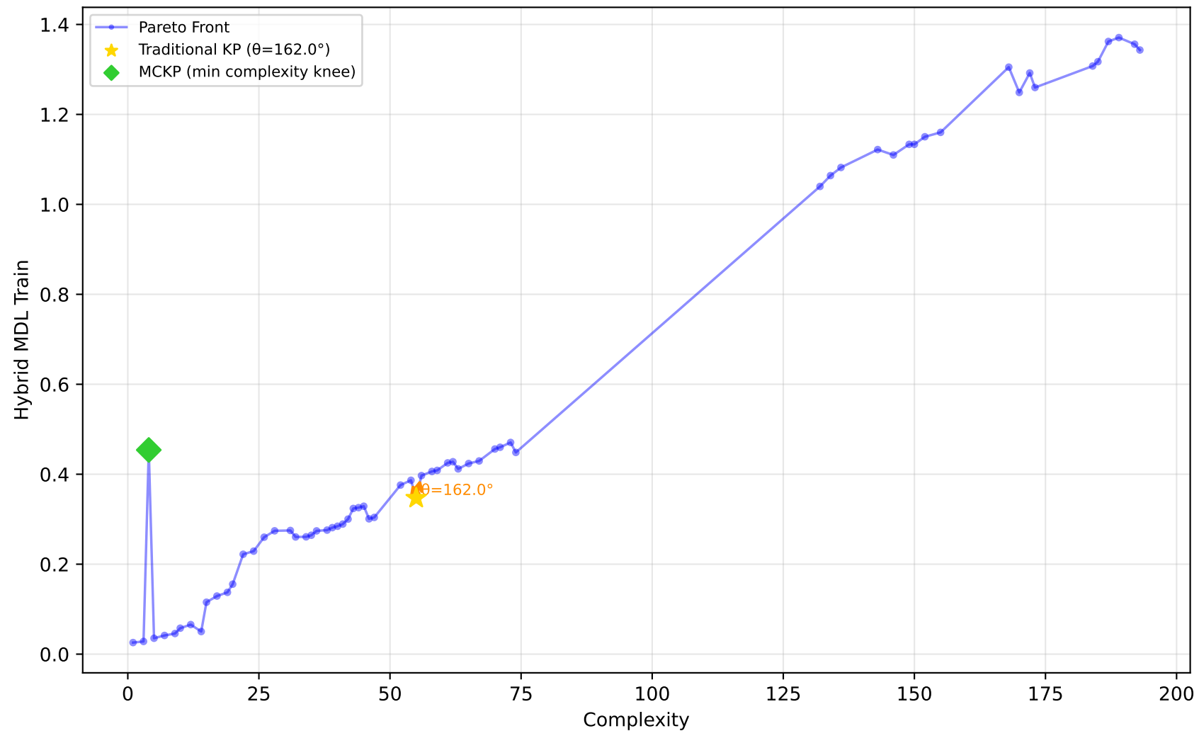
228_elusage - Run 20 - SVP - Hybrid MDL Train \lambda_1=0.00, \bar{\lambda}_2=1.00, \lambda_3=0.00 | Difficulty: 1.00 | Method: hmr
