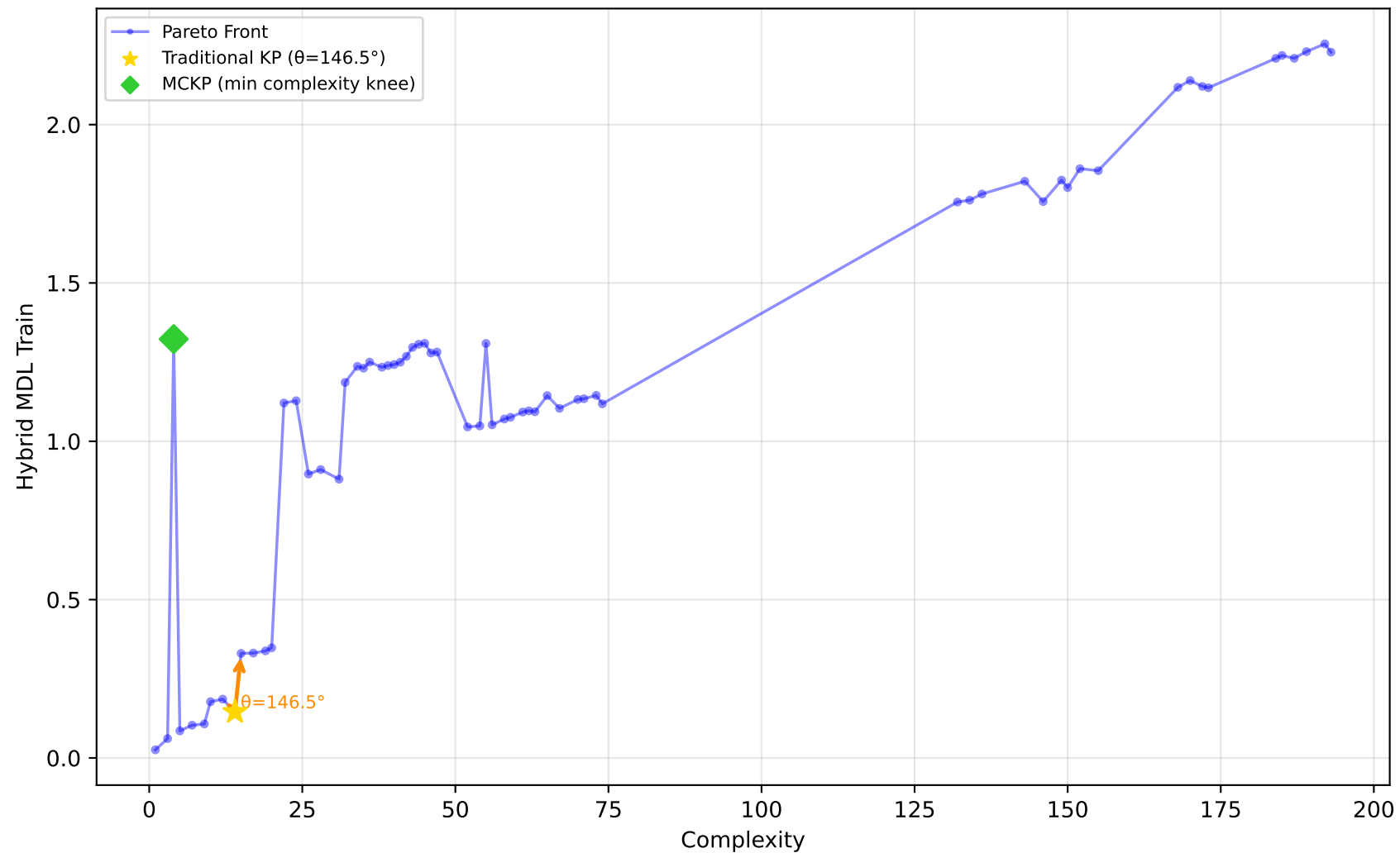
228_elusage - Run 20 - SVP - Hybrid MDL Train \lambda_1=0.60, \bar{\lambda}_2=0.60, \lambda_3=1.00 | Difficulty: 1.00 | Method: hmr
