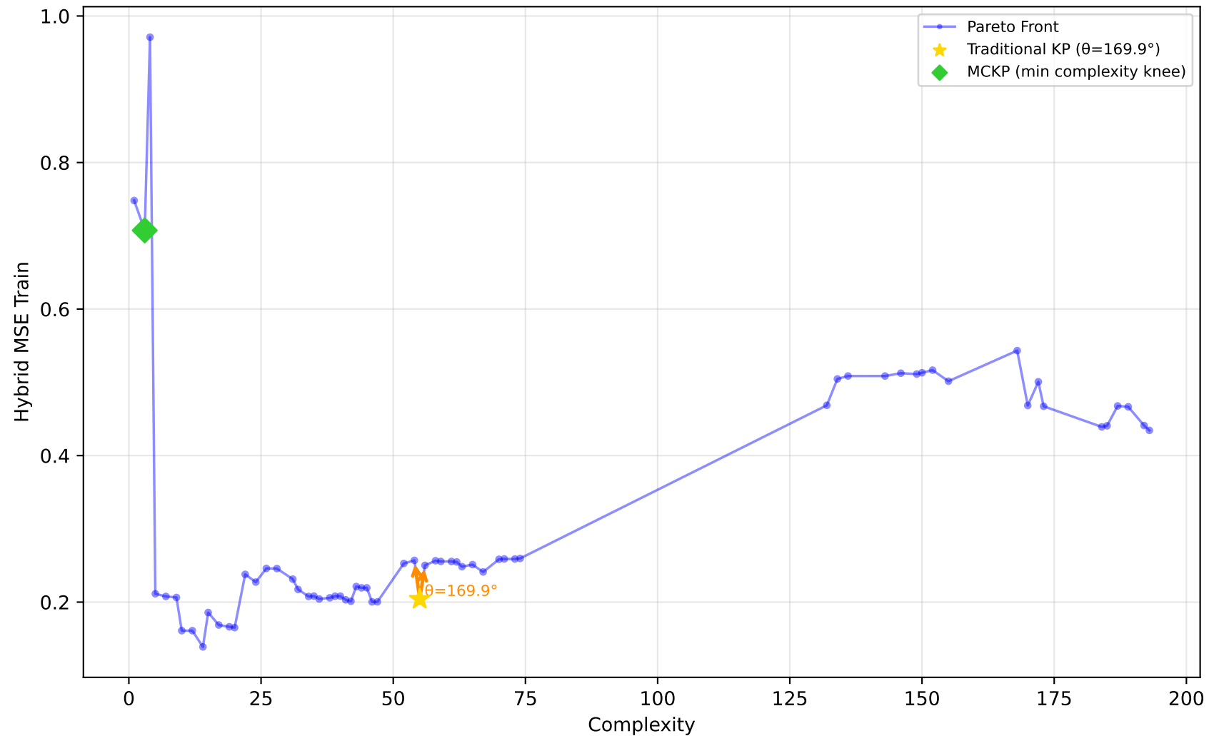
228_elusage - Run 20 - SVP - Hybrid MSE Train \lambda_1=0.00, \bar{\lambda}_2=1.00, \lambda_3=0.00 | Difficulty: 1.00 | Method: hmr
