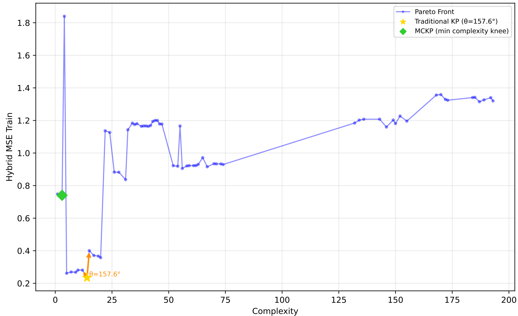
228_elusage - Run 20 - SVP - Hybrid MSE Train \lambda_1=0.60, \bar{\lambda}_2=0.60, \lambda_3=1.00 | Difficulty: 1.00 | Method: hmr
