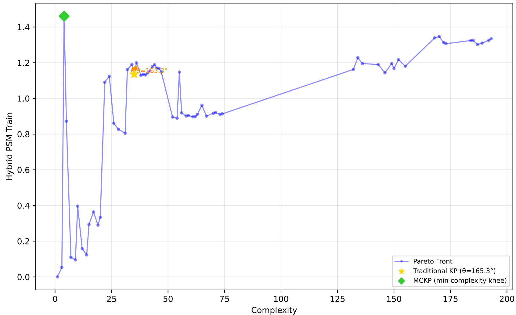
228_elusage - Run 20 - SVP - Hybrid PSM Train \lambda_1=0.60, \bar{\lambda}_2=0.60, \lambda_3=1.00 | Difficulty: 1.00 | Method: hmr
