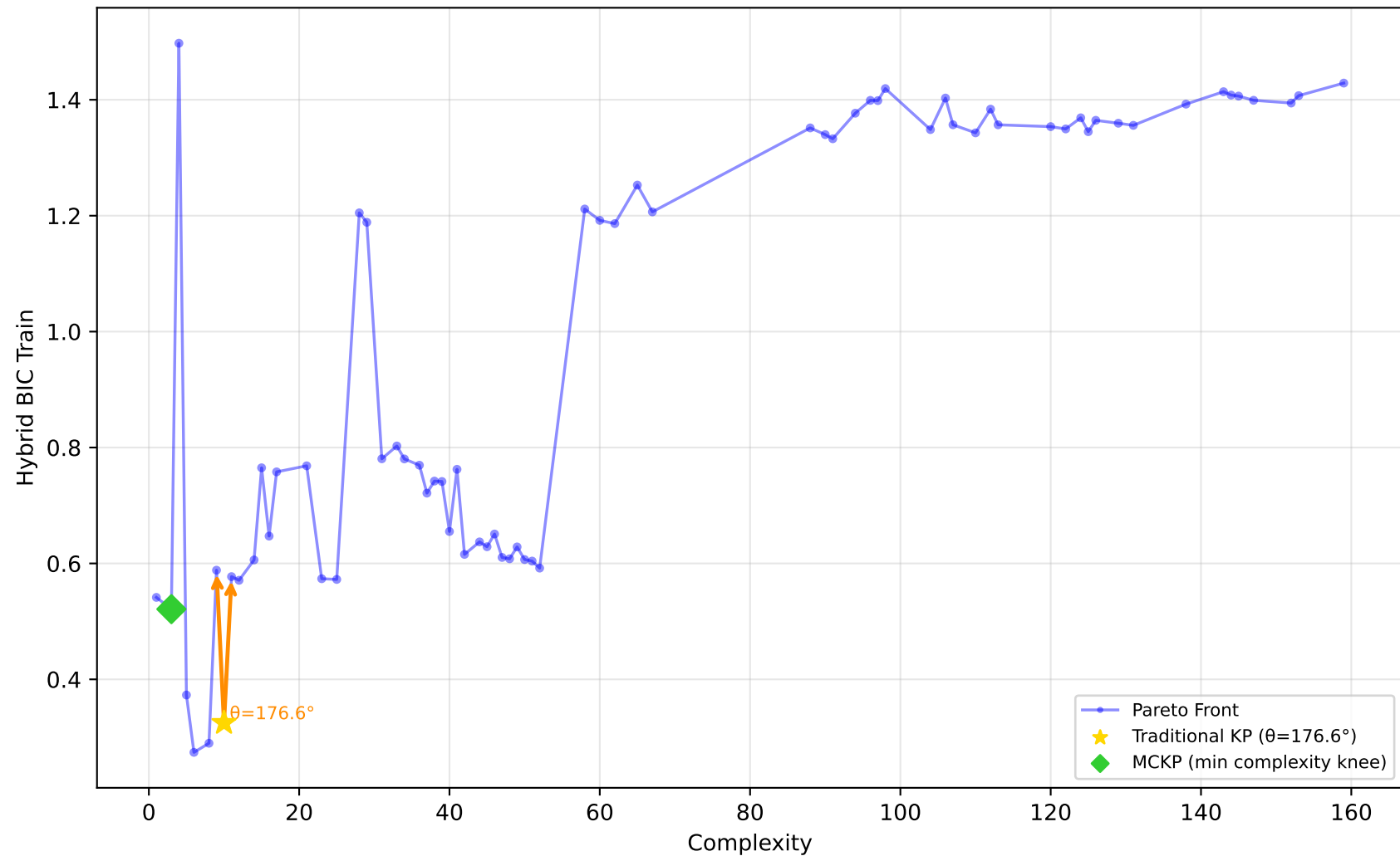
228_elusage - Run 21 - MVP - Hybrid BIC Train \lambda_1=0.00 , \lambda_2=0.00 , \lambda_3=1.00 | Difficulty: 0.67 | Method: hmr
