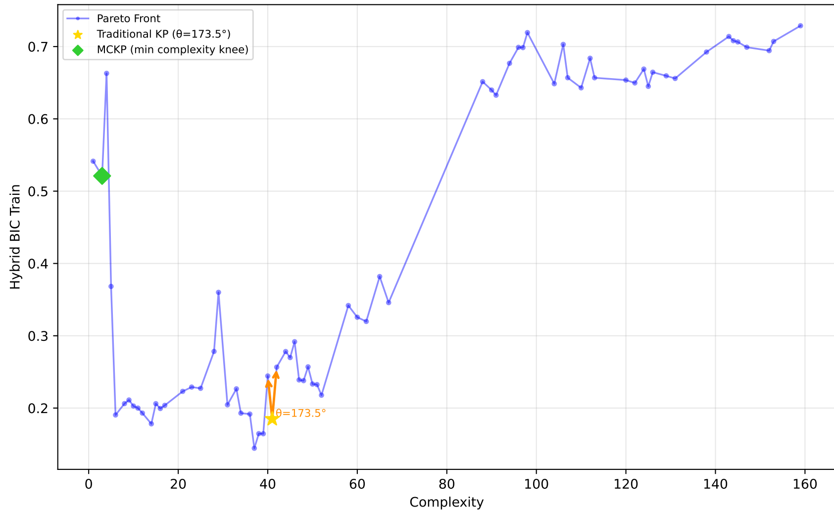
228_elusage - Run 21 - MVP - Hybrid BIC Train \lambda_1=0.00, \lambda_2=0.30, \lambda_3=0.00 | Difficulty: 0.67 | Method: hmr
