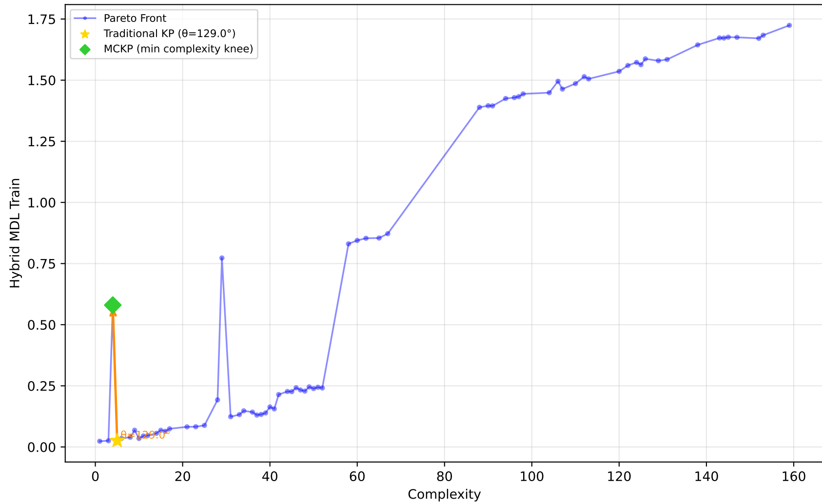
228_elusage - Run 21 - SVP - Hybrid MDL Train \lambda_1=0.00 , \bar{\lambda}_2=1.00 , \lambda_3=0.00 | Difficulty: 0.67 | Method: hmr
