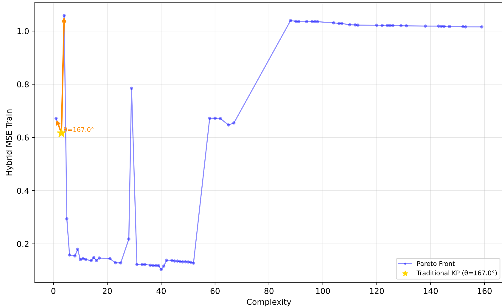
228_elusage - Run 21 - SVP - Hybrid MSE Train \lambda_1=0.00, \bar{\lambda}_2=1.00, \lambda_3=0.00 | Difficulty: 0.67 | Method: hmr
