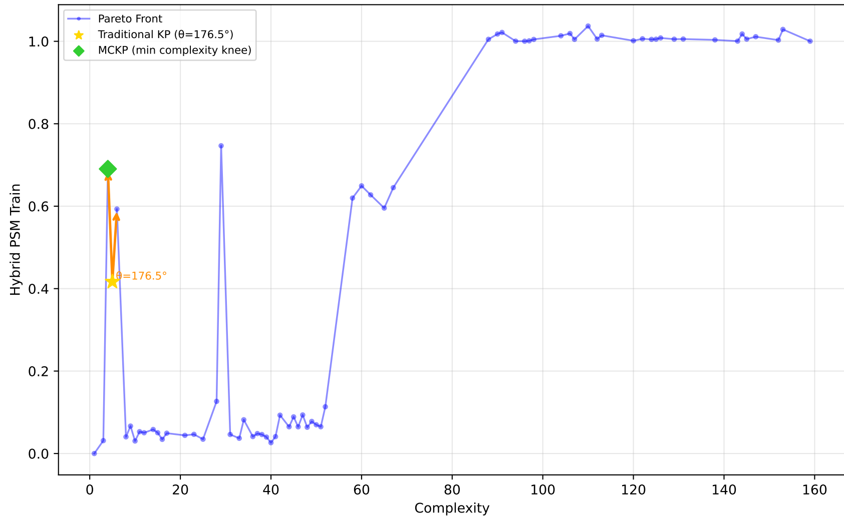
228_elusage - Run 21 - SVP - Hybrid PSM Train \lambda_1=0.00, \bar{\lambda}_2=1.00, \lambda_3=0.00 | Difficulty: 0.67 | Method: hmr
