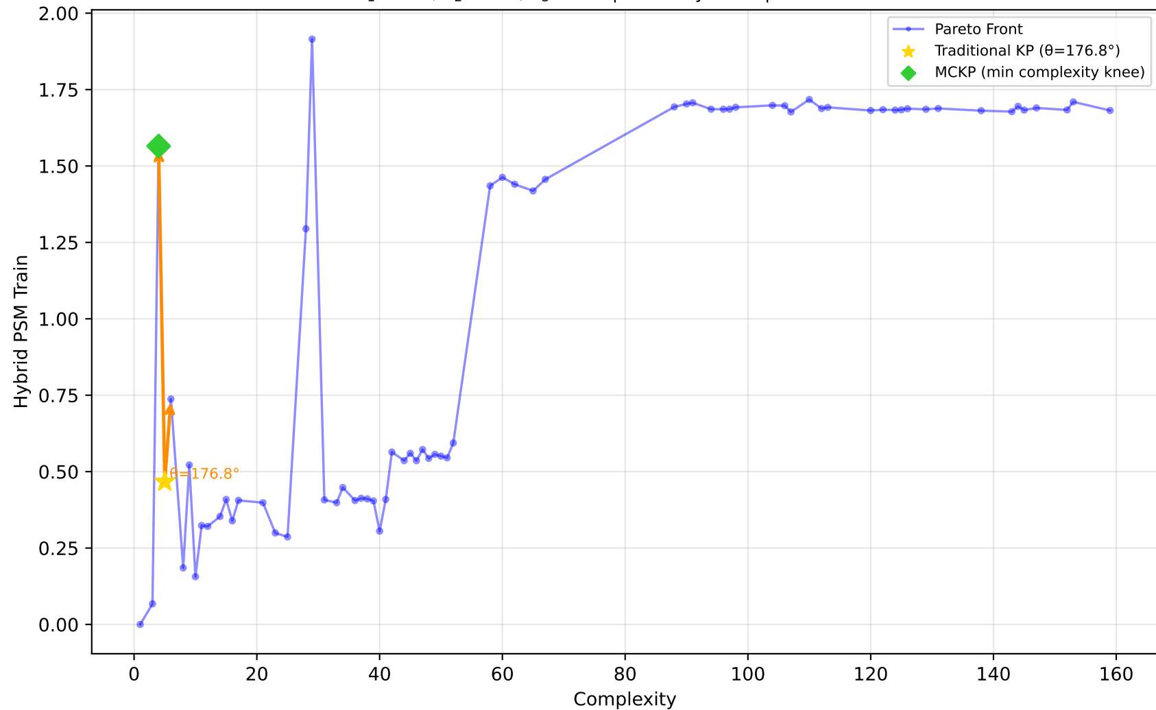
228_elusage - Run 21 - SVP - Hybrid PSM Train \lambda_1=0.60, \bar{\lambda}_2=0.60, \lambda_3=1.00 | Difficulty: 0.67 | Method: hmr
