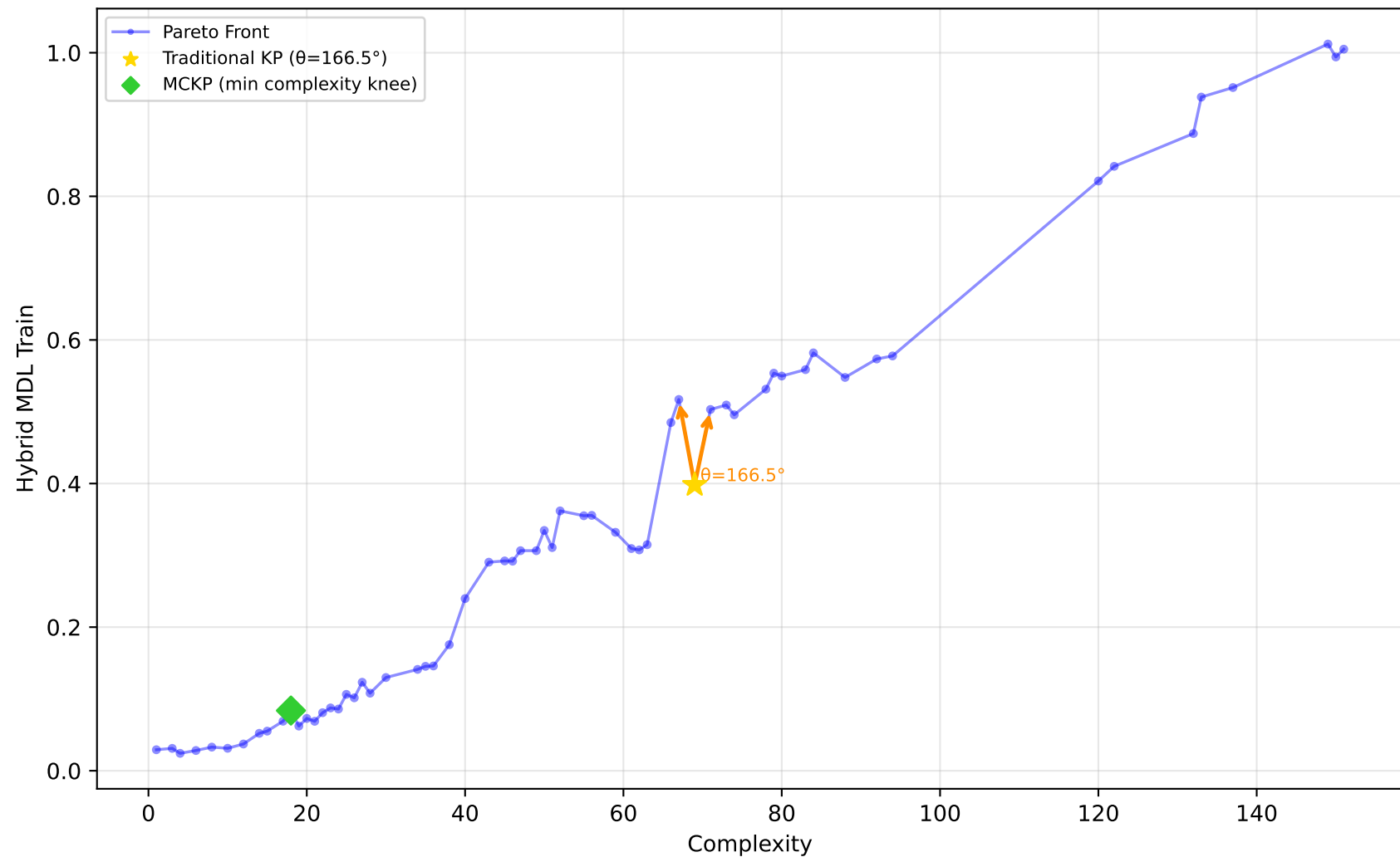
228_elusage - Run 22 - MVP - Hybrid MDL Train \lambda_1=0.00, \bar{\lambda}_2=0.30, \lambda_3=0.00 | Difficulty: 1.00 | Method: hmr
