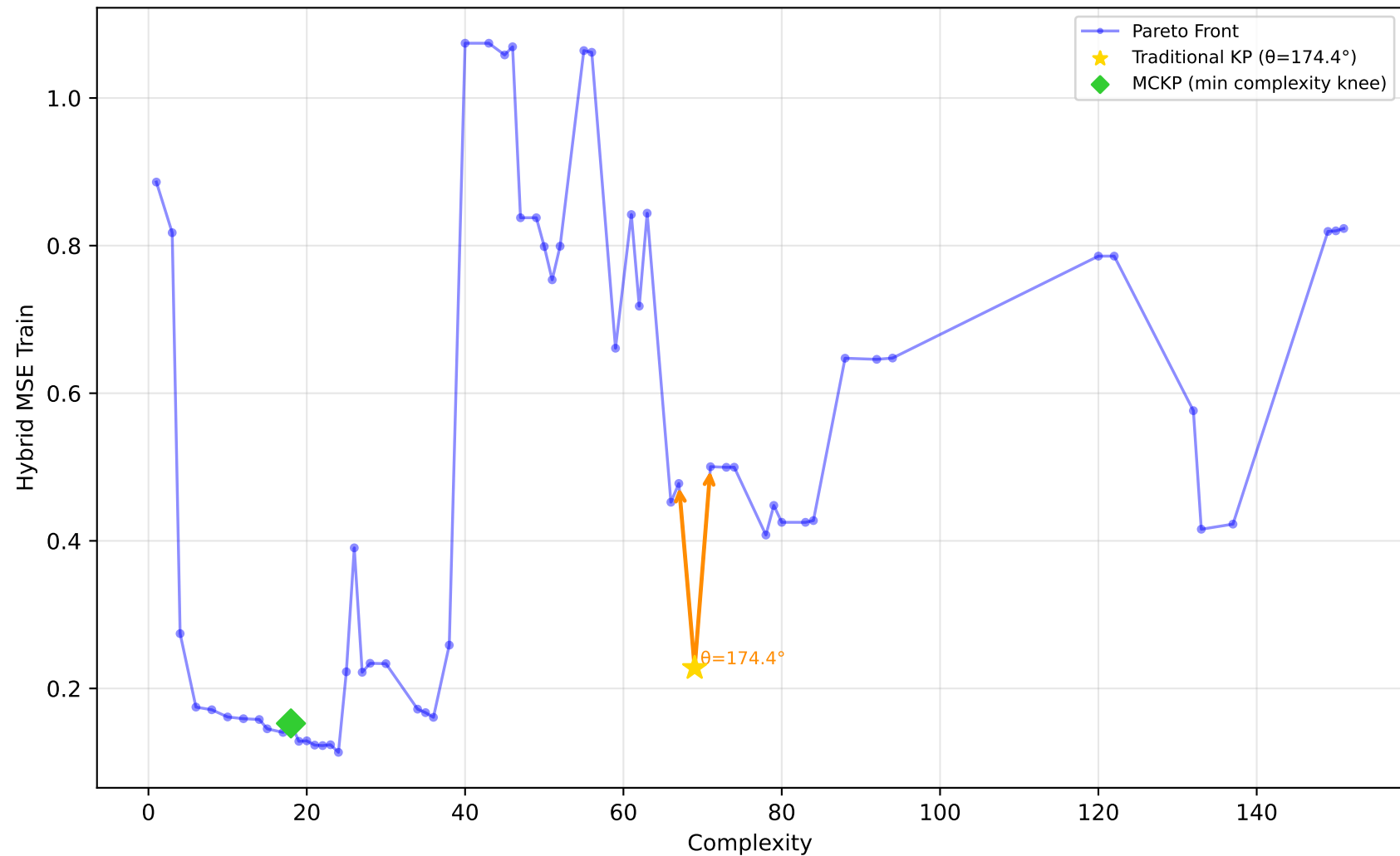
228_elusage - Run 22 - MVP - Hybrid MSE Train \lambda_1=0.00, \bar{\lambda}_2=0.00, \lambda_3=1.00 | Difficulty: 1.00 | Method: hmr
