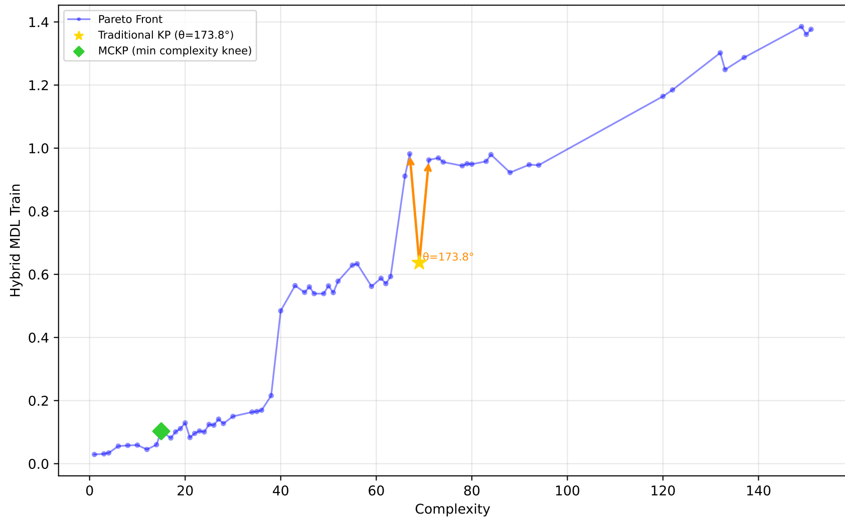
228_elusage - Run 22 - SVP - Hybrid MDL Train \lambda_1=0.00, \bar{\lambda}_2=1.00, \lambda_3=0.00 | Difficulty: 1.00 | Method: hmr
