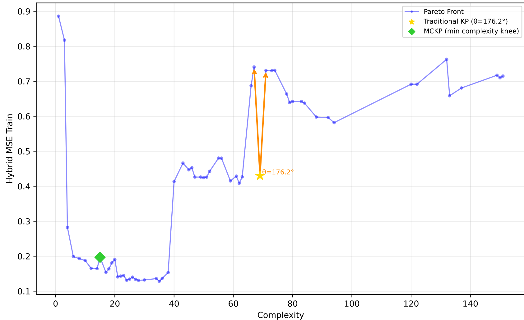
228_elusage - Run 22 - SVP - Hybrid MSE Train \lambda_1=0.00, \bar{\lambda}_2=1.00, \lambda_3=0.00 | Difficulty: 1.00 | Method: hmr
