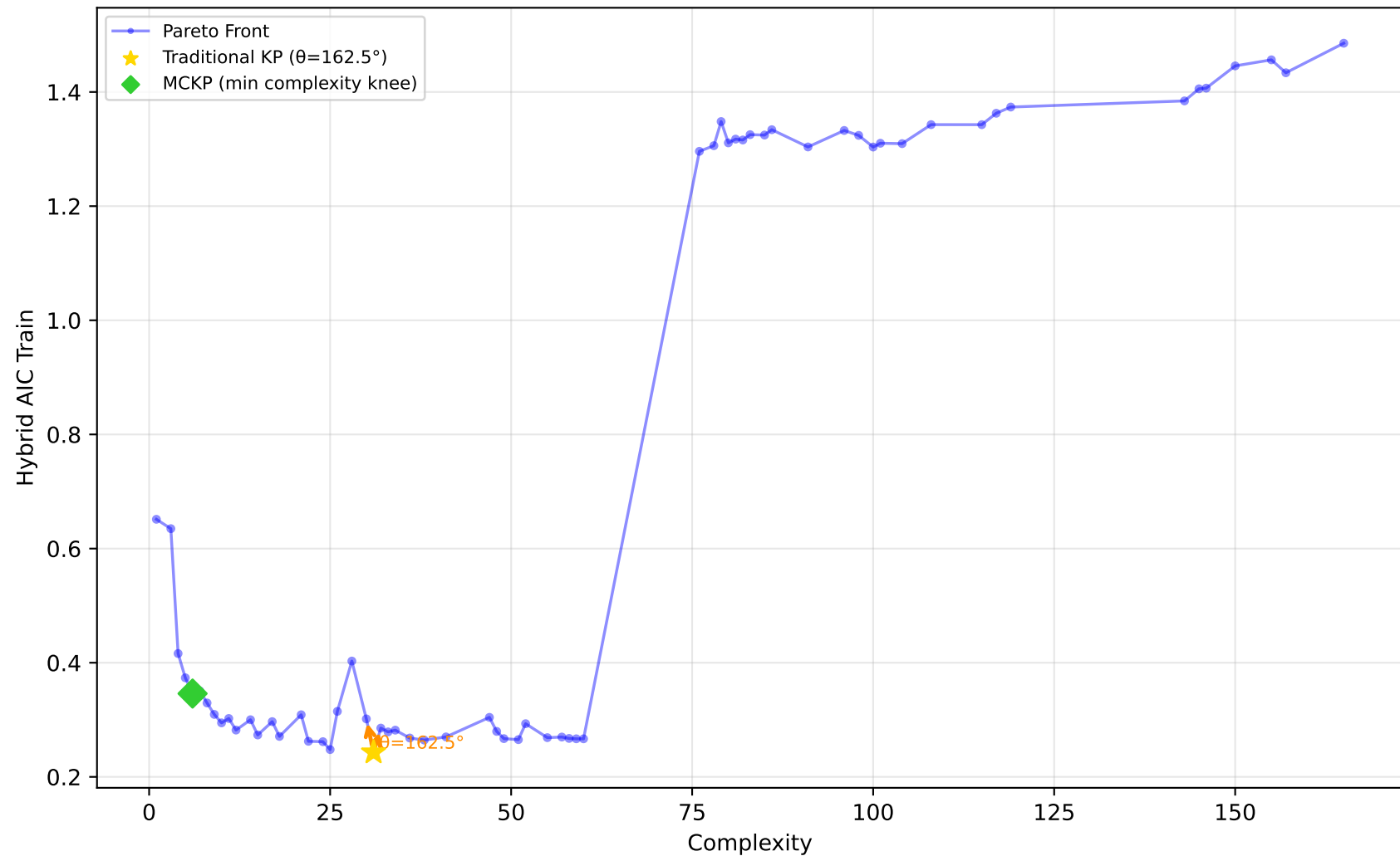
228_elusage - Run 23 - MVP - Hybrid AIC Train \lambda_1=0.00, \lambda_2=0.00, \lambda_3=1.00 | Difficulty: 1.00 | Method: hmr
