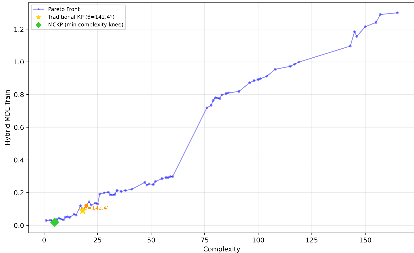
228_elusage - Run 23 - MVP - Hybrid MDL Train \lambda_1=0.00, \bar{\lambda}_2=0.30, \lambda_3=0.00 | Difficulty: 1.00 | Method: hmr
