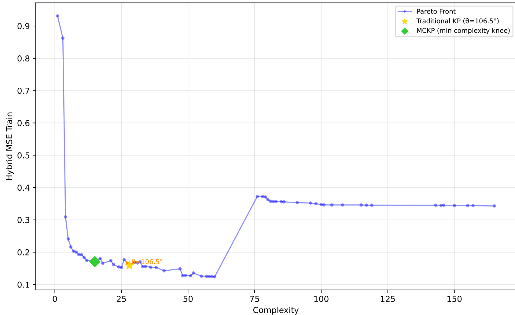
228_elusage - Run 23 - MVP - Hybrid MSE Train \lambda_1=0.00, \bar{\lambda}_2=0.30, \lambda_3=0.00 | Difficulty: 1.00 | Method: hmr
