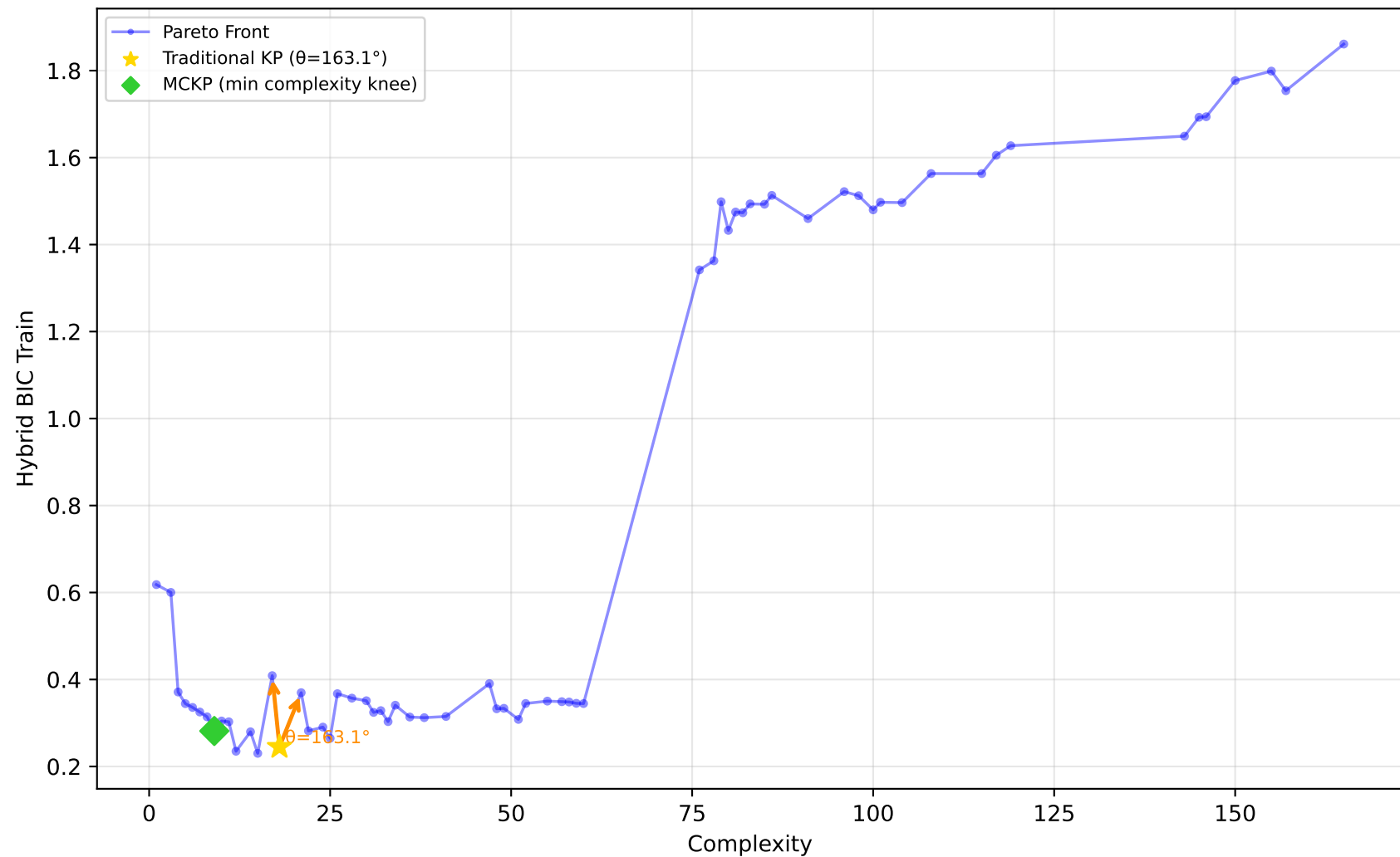
228_elusage - Run 23 - SVP - Hybrid BIC Train \lambda_1=0.00, \lambda_2=1.00, \lambda_3=0.00 | Difficulty: 1.00 | Method: hmr
