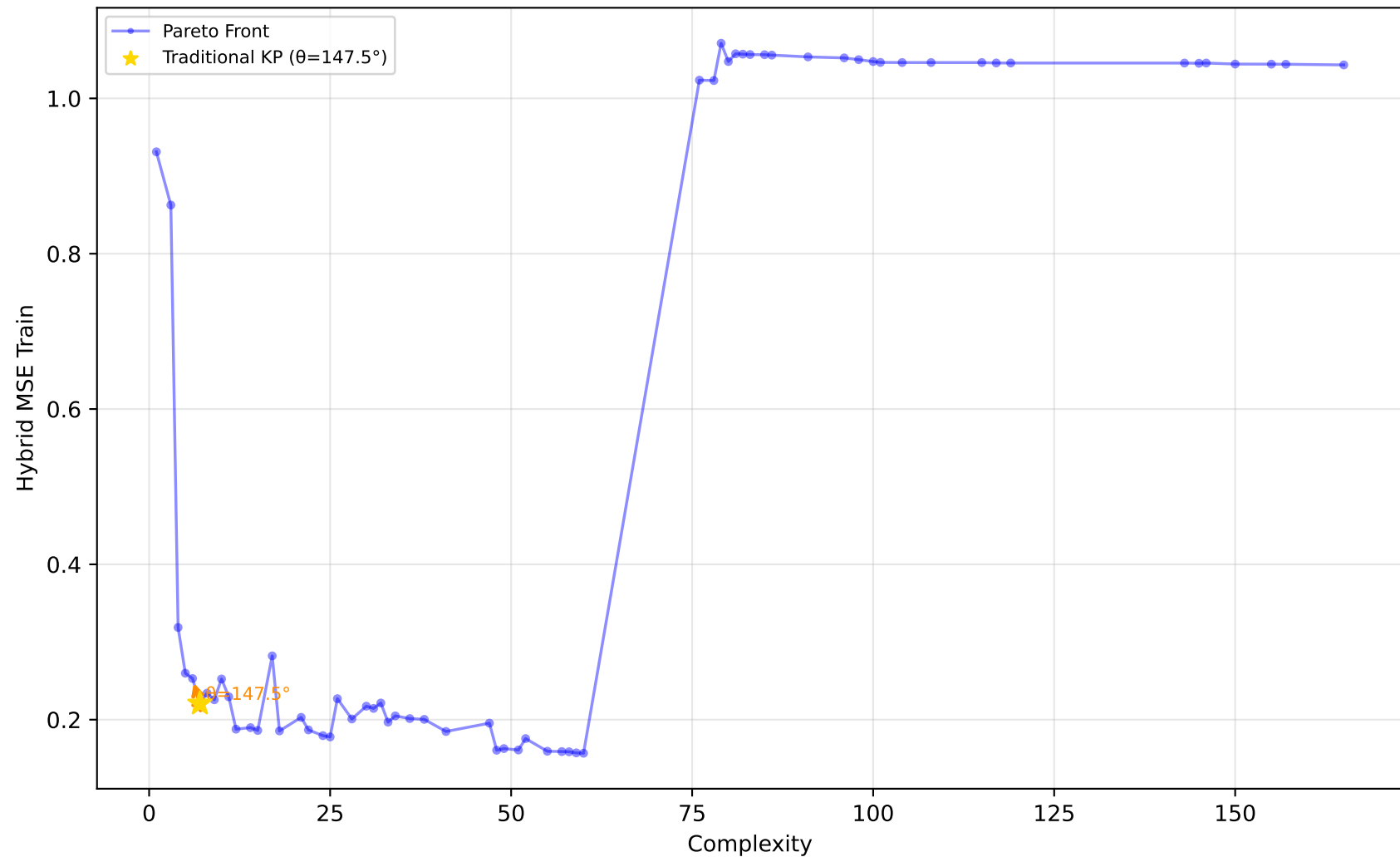
228_elusage - Run 23 - SVP - Hybrid MSE Train \lambda_1=0.00, \bar{\lambda}_2=1.00, \lambda_3=0.00 | Difficulty: 1.00 | Method: hmr
