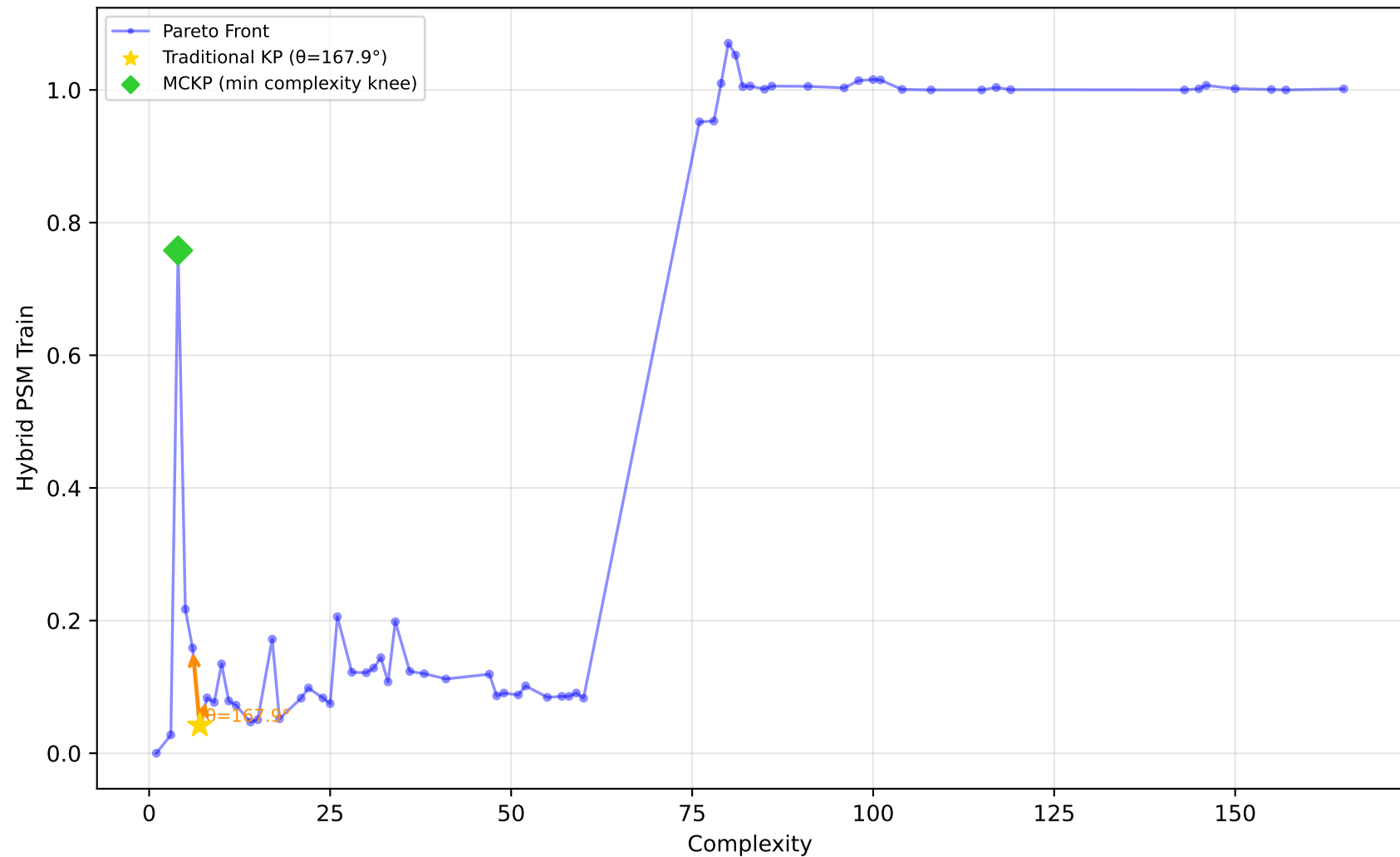
228_elusage - Run 23 - SVP - Hybrid PSM Train \lambda_1=0.00, \bar{\lambda}_2=1.00, \lambda_3=0.00 | Difficulty: 1.00 | Method: hmr
