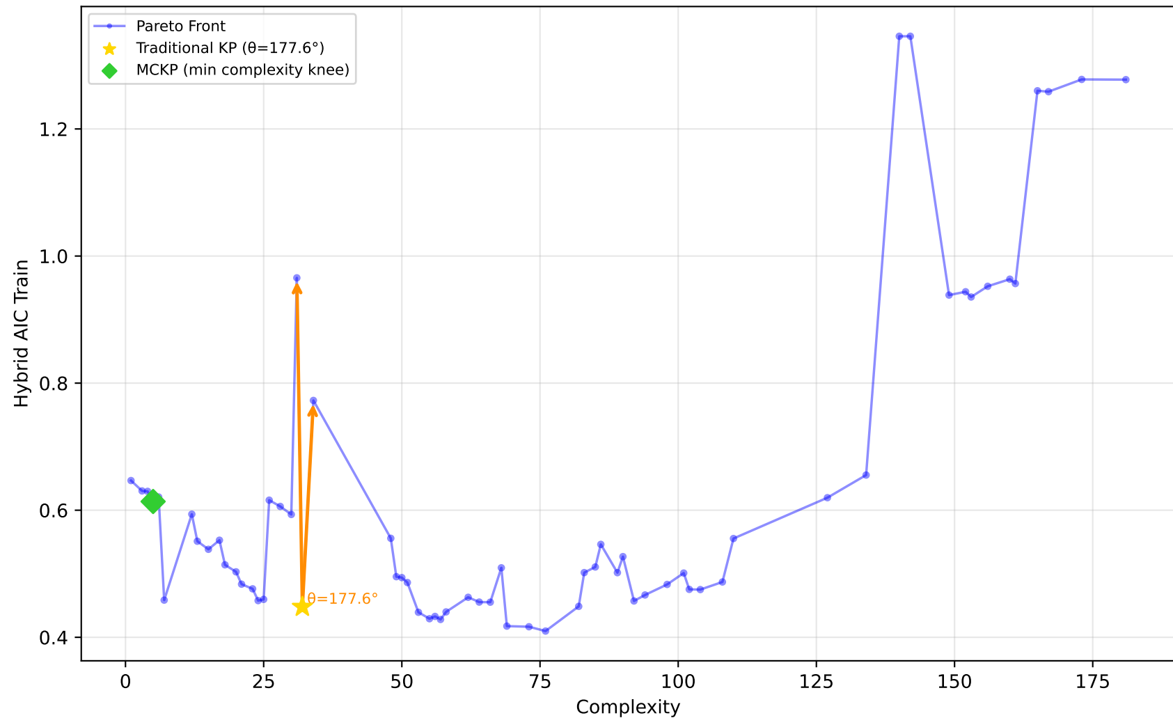
228_elusage - Run 24 - MVP - Hybrid AIC Train \lambda_1=0.00, \lambda_2=0.00, \lambda_3=1.00 | Difficulty: 1.00 | Method: hmr
