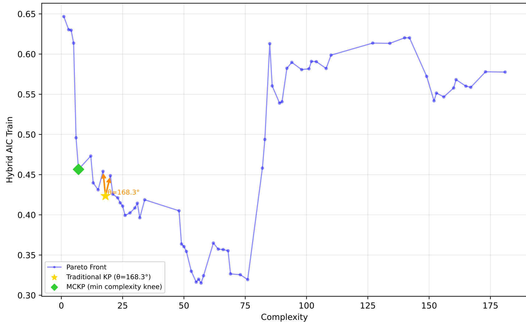
228_elusage - Run 24 - MVP - Hybrid AIC Train \lambda_1=0.00, \bar{\lambda}_2=0.30, \lambda_3=0.00 | Difficulty: 1.00 | Method: hmr
