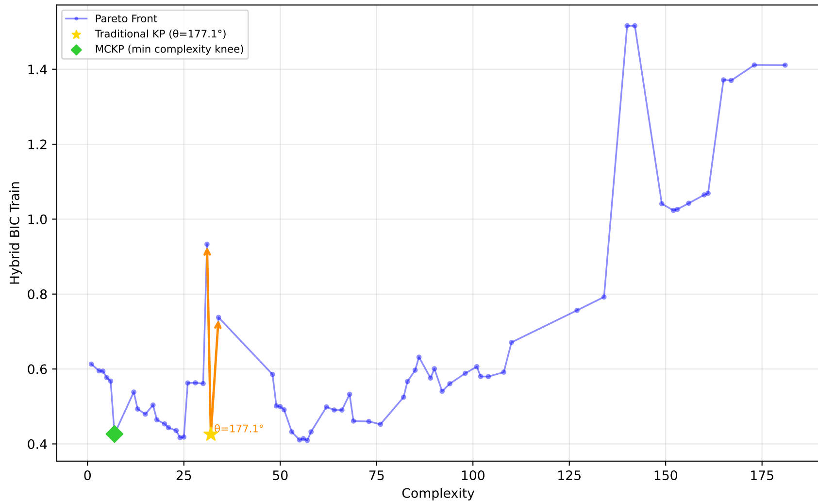
228_elusage - Run 24 - MVP - Hybrid BIC Train \lambda_1=0.00, \lambda_2=0.00, \lambda_3=1.00 | Difficulty: 1.00 | Method: hmr
