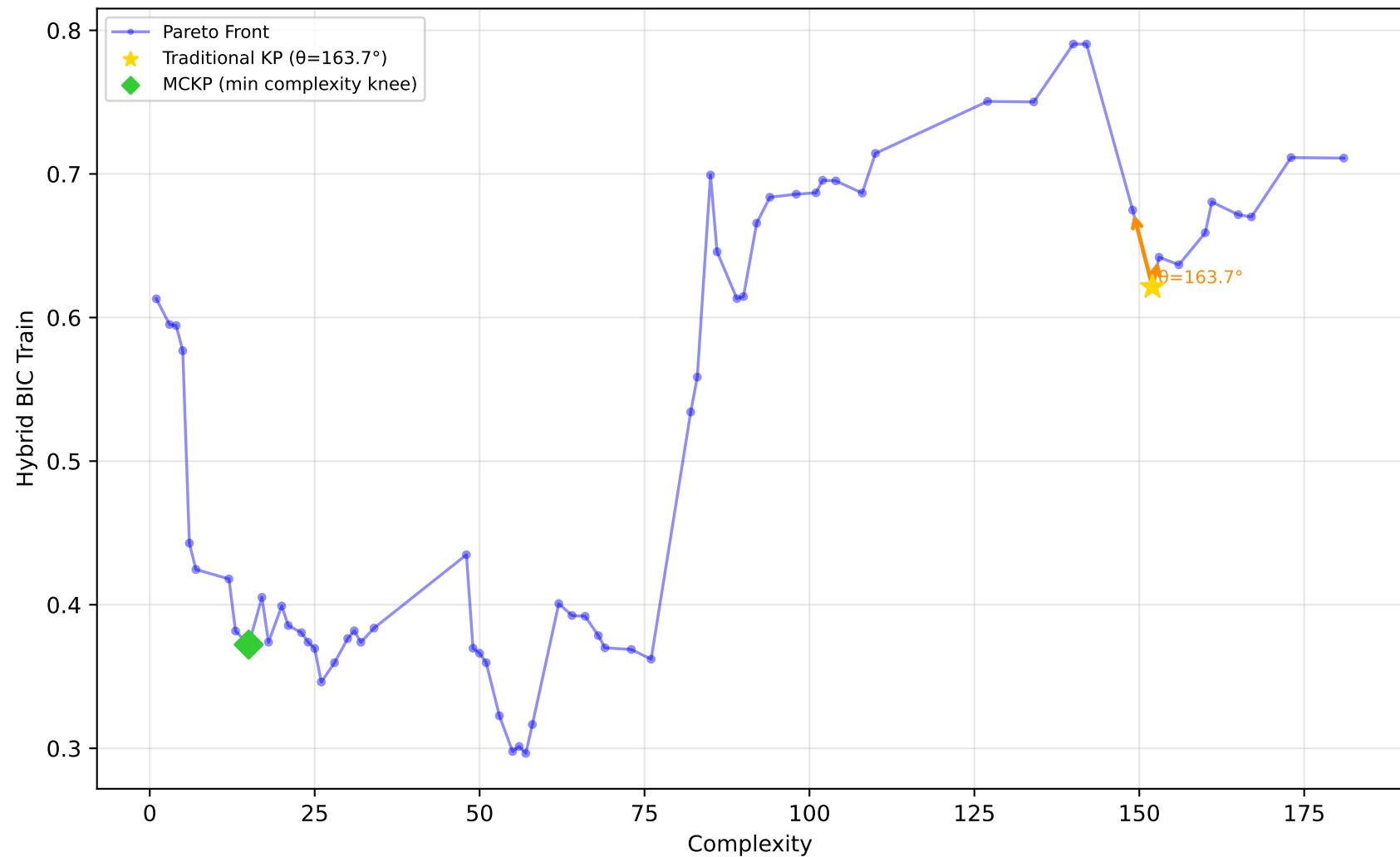
228_elusage - Run 24 - MVP - Hybrid BIC Train \lambda_1=0.00, \lambda_2=0.30, \lambda_3=0.00 | Difficulty: 1.00 | Method: hmr
