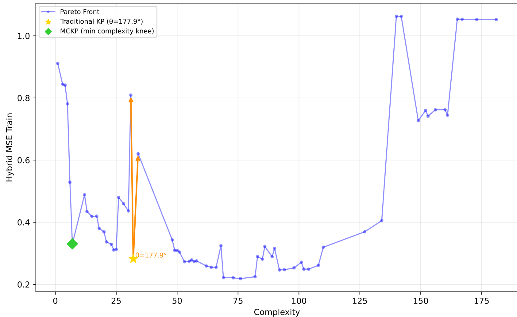
228_elusage - Run 24 - MVP - Hybrid MSE Train \lambda_1=0.00, \bar{\lambda}_2=0.00, \lambda_3=1.00 | Difficulty: 1.00 | Method: hmr
