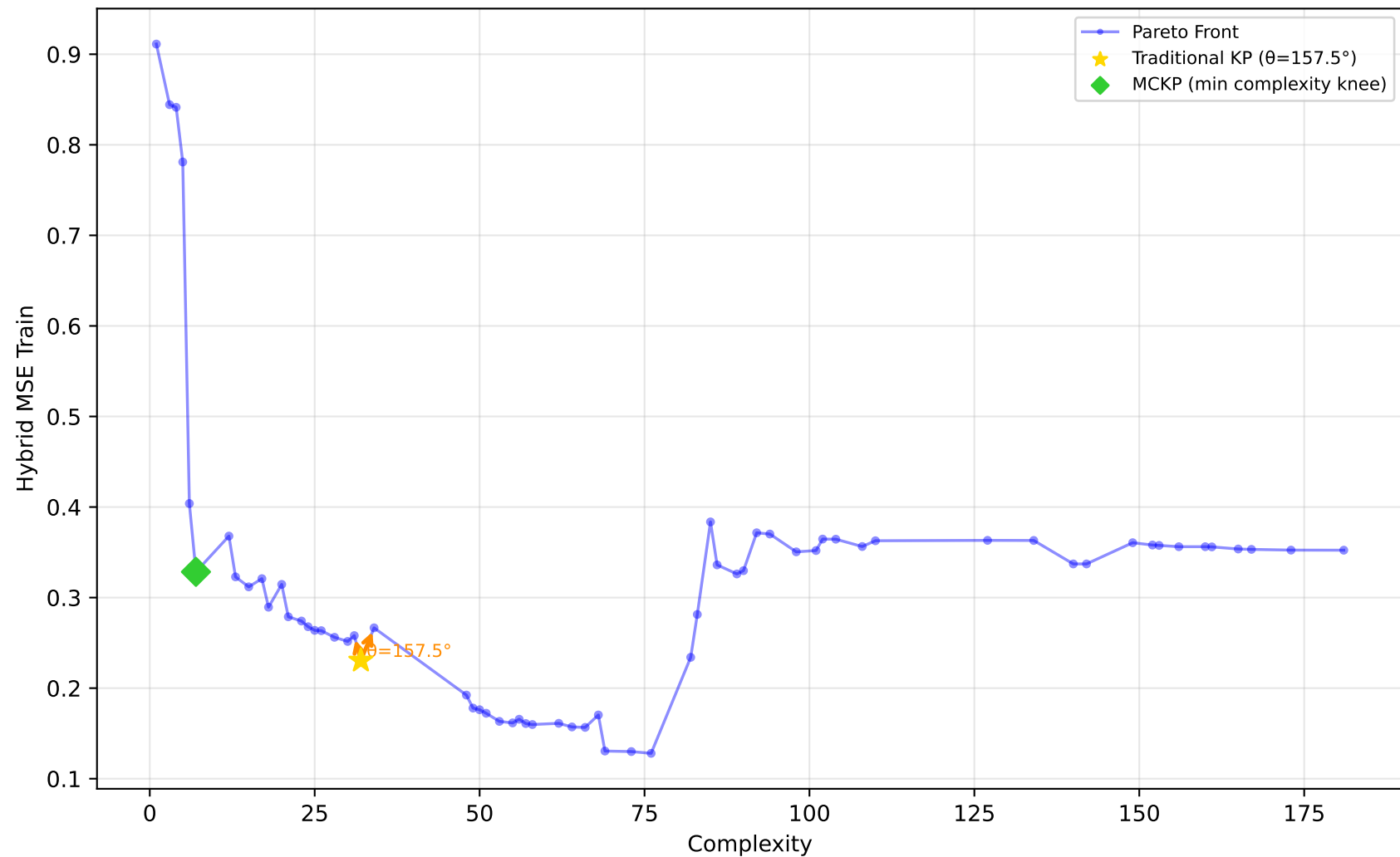
228_elusage - Run 24 - MVP - Hybrid MSE Train \lambda_1=0.00, \bar{\lambda}_2=0.30, \lambda_3=0.00 | Difficulty: 1.00 | Method: hmr
