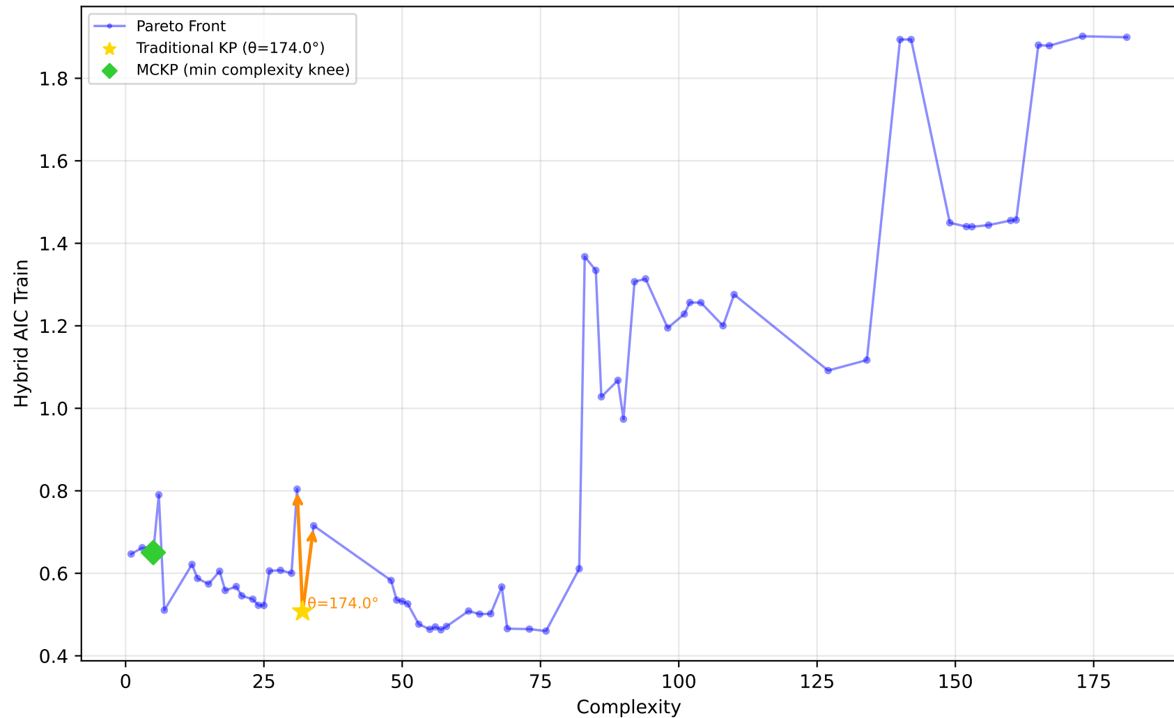
228_elusage - Run 24 - SVP - Hybrid AIC Train \lambda_1=0.60, \lambda_2=0.60, \lambda_3=1.00 | Difficulty: 1.00 | Method: hmr
