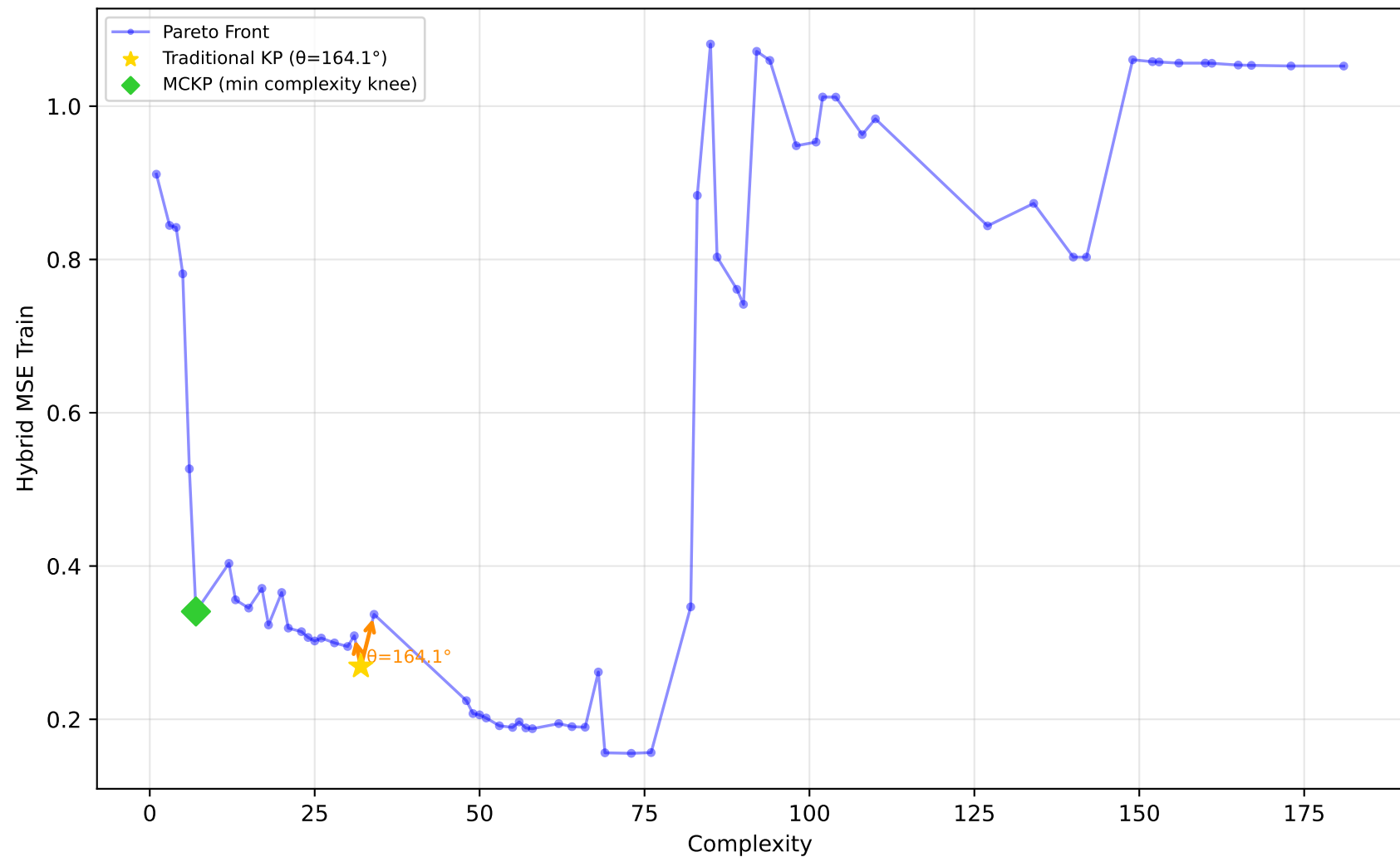
228_elusage - Run 24 - SVP - Hybrid MSE Train \lambda_1=0.00, \bar{\lambda}_2=1.00, \lambda_3=0.00 | Difficulty: 1.00 | Method: hmr
