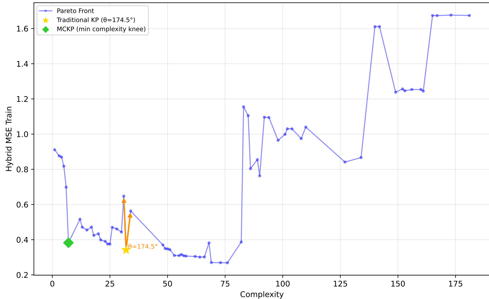
228_elusage - Run 24 - SVP - Hybrid MSE Train \lambda_1=0.60, \bar{\lambda}_2=0.60, \lambda_3=1.00 | Difficulty: 1.00 | Method: hmr
