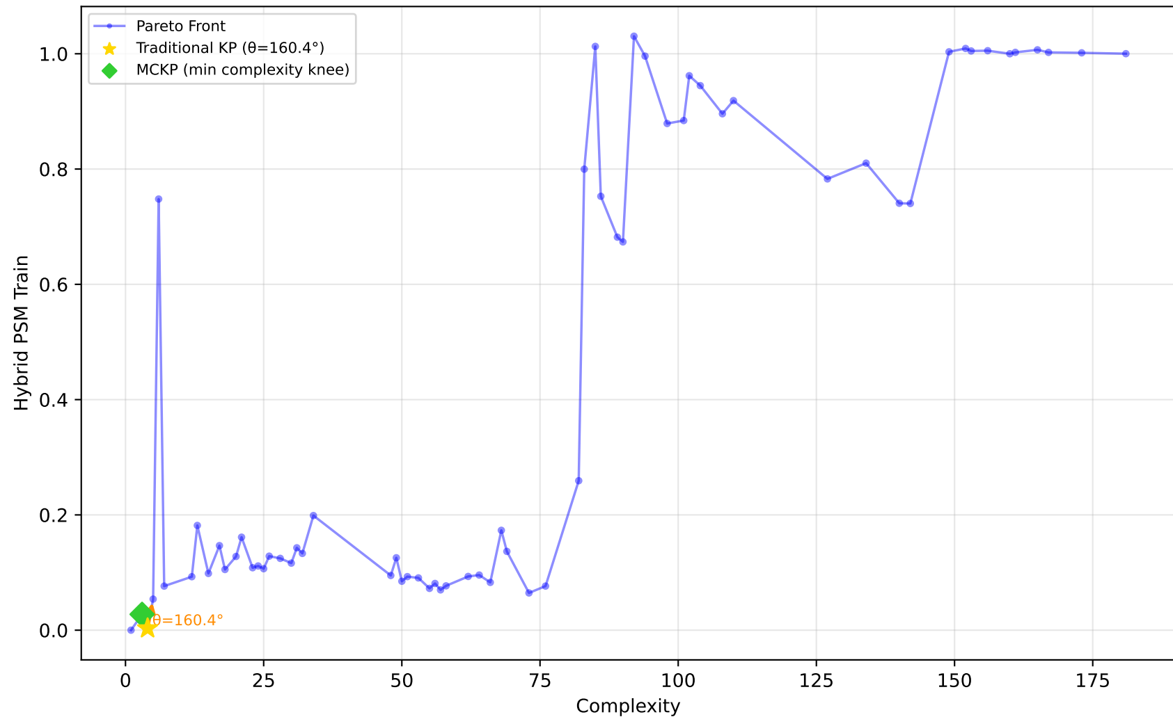
228_elusage - Run 24 - SVP - Hybrid PSM Train \lambda_1=0.00, \lambda_2=1.00, \lambda_3=0.00 | Difficulty: 1.00 | Method: hmr
