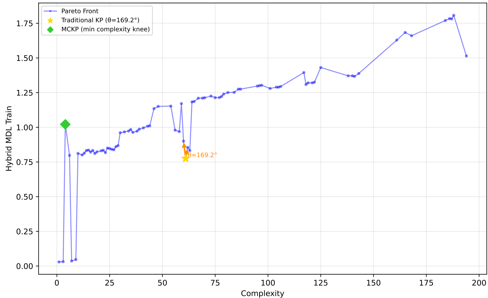
228 elusage - Run 25 - MVP - Hybrid MDL Train \lambda_1=0.00 , \bar{\lambda}_2=0.00 , \lambda_3=1.00 | Difficulty: 0.87 | Method: hmr
