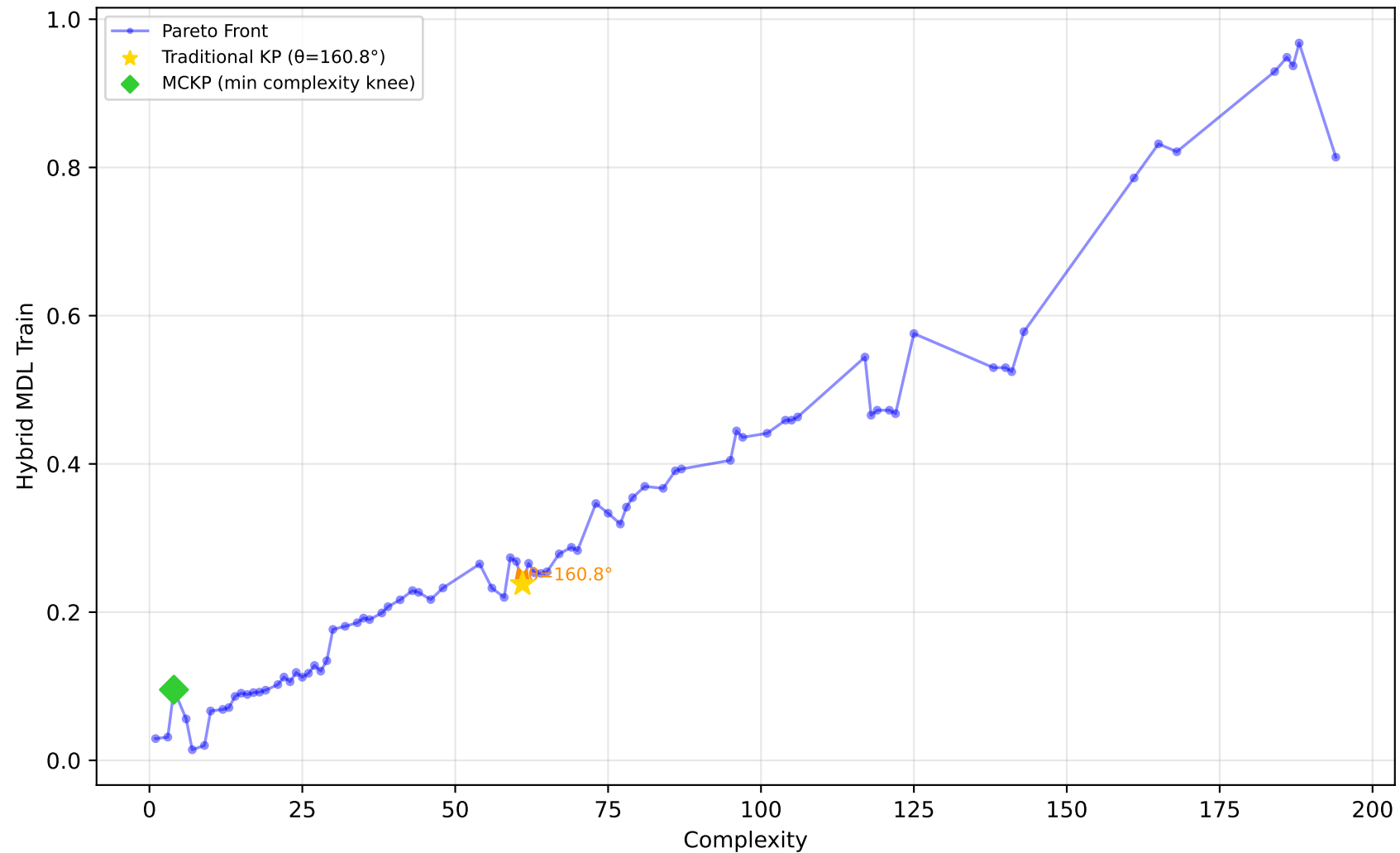
228_elusage - Run 25 - MVP - Hybrid MDL Train \lambda_1=0.00, \bar{\lambda}_2=0.30, \lambda_3=0.00 | Difficulty: 0.87 | Method: hmr
