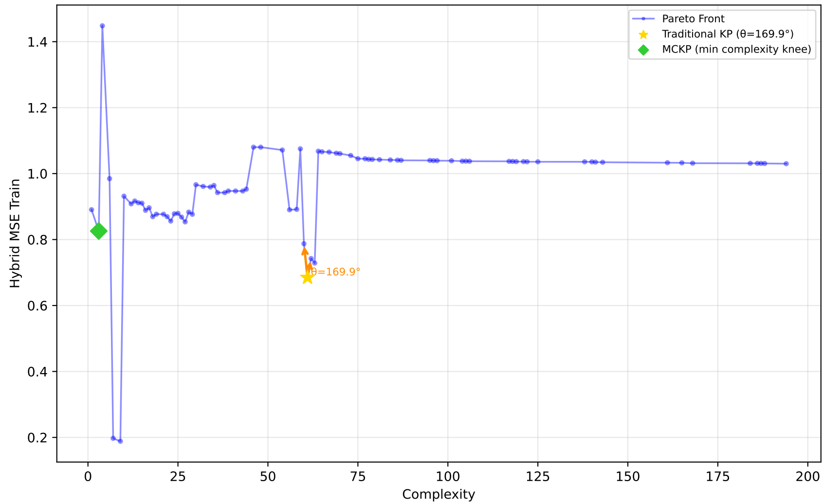
228_elusage - Run 25 - MVP - Hybrid MSE Train \lambda_1=0.00, \bar{\lambda}_2=0.00, \lambda_3=1.00 | Difficulty: 0.87 | Method: hmr
