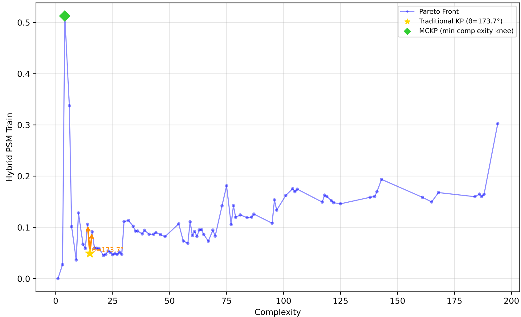
228_elusage - Run 25 - MVP - Hybrid PSM Train \lambda_1=0.00, \bar{\lambda}_2=0.30, \lambda_3=0.00 | Difficulty: 0.87 | Method: hmr
