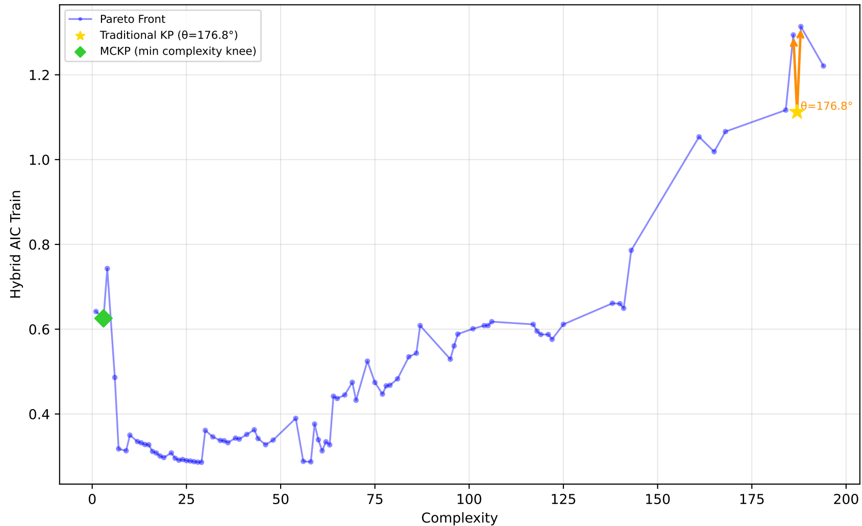
228_elusage - Run 25 - SVP - Hybrid AIC Train \lambda_1=0.00, \lambda_2=1.00, \lambda_3=0.00 | Difficulty: 0.87 | Method: hmr
