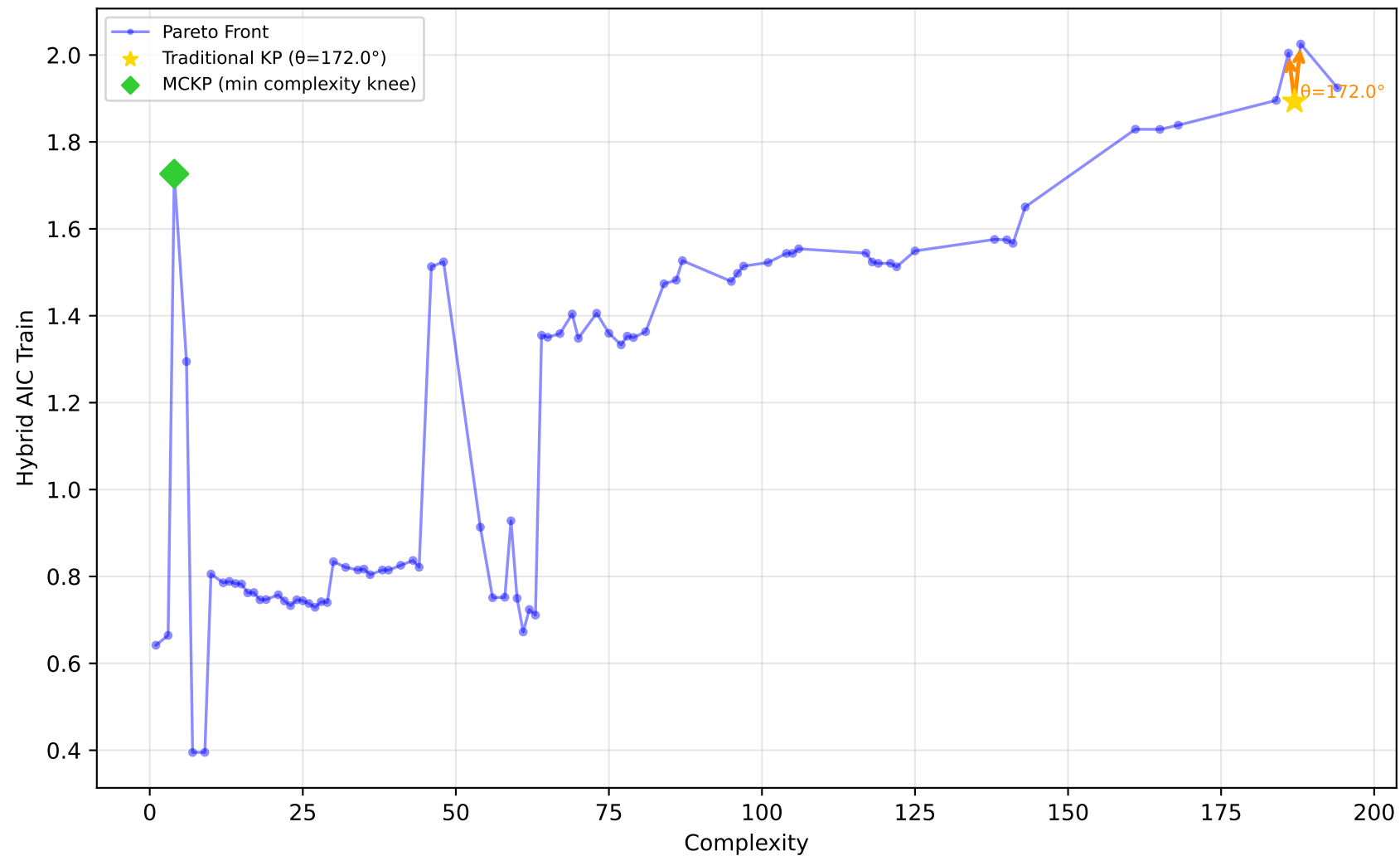
228_elusage - Run 25 - SVP - Hybrid AIC Train \lambda_1=0.60, \lambda_2=0.60, \lambda_3=1.00 | Difficulty: 0.87 | Method: hmr
