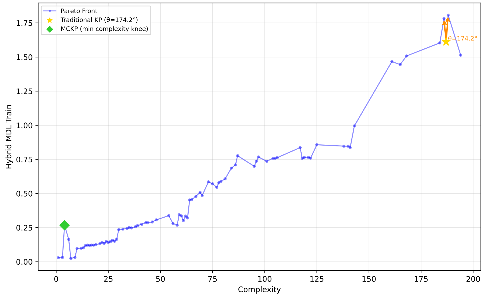
228_elusage - Run 25 - SVP - Hybrid MDL Train \lambda_1=0.00, \bar{\lambda}_2=1.00, \lambda_3=0.00 | Difficulty: 0.87 | Method: hmr
