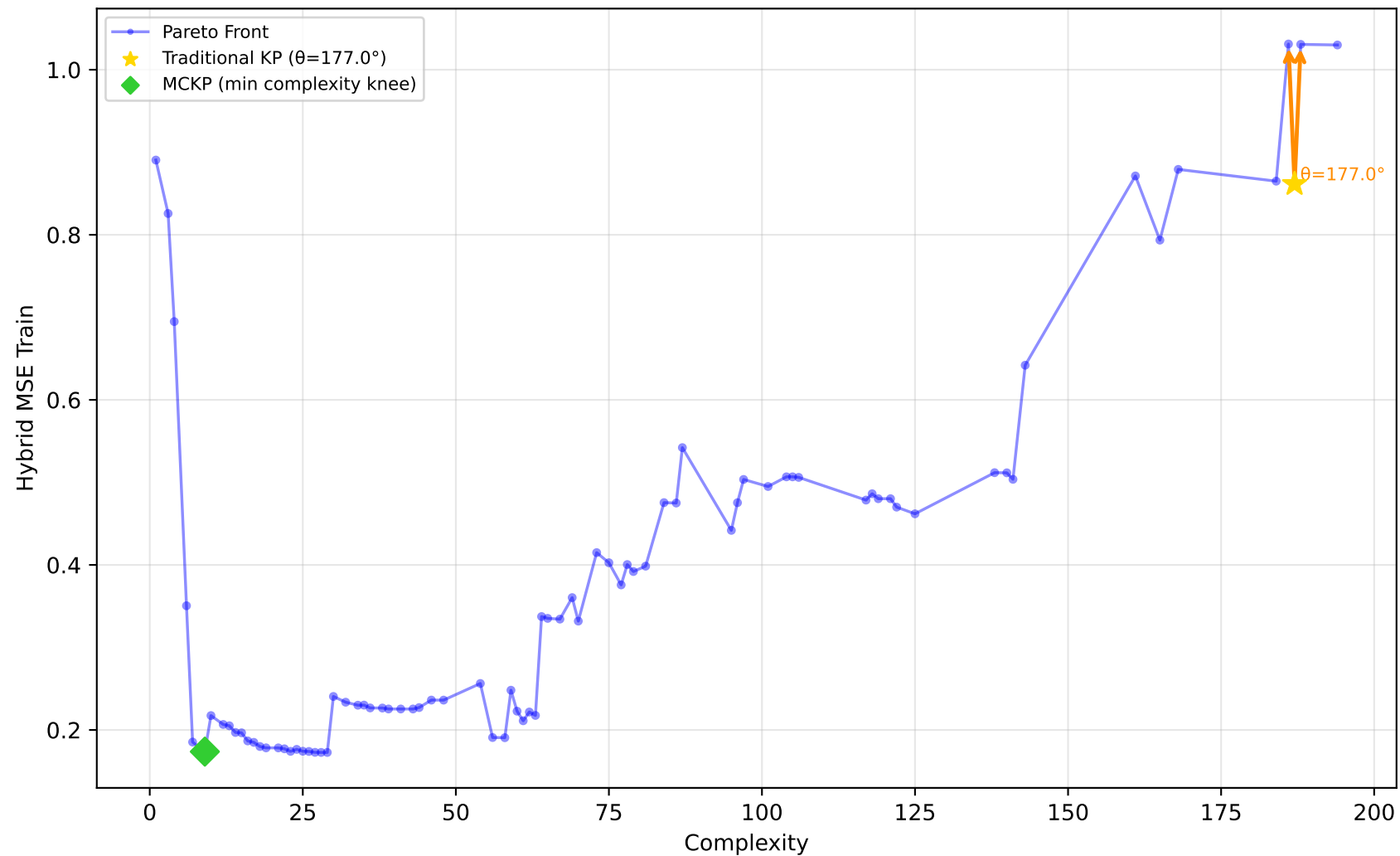
228_elusage - Run 25 - SVP - Hybrid MSE Train \lambda_1=0.00, \bar{\lambda}_2=1.00, \lambda_3=0.00 | Difficulty: 0.87 | Method: hmr
