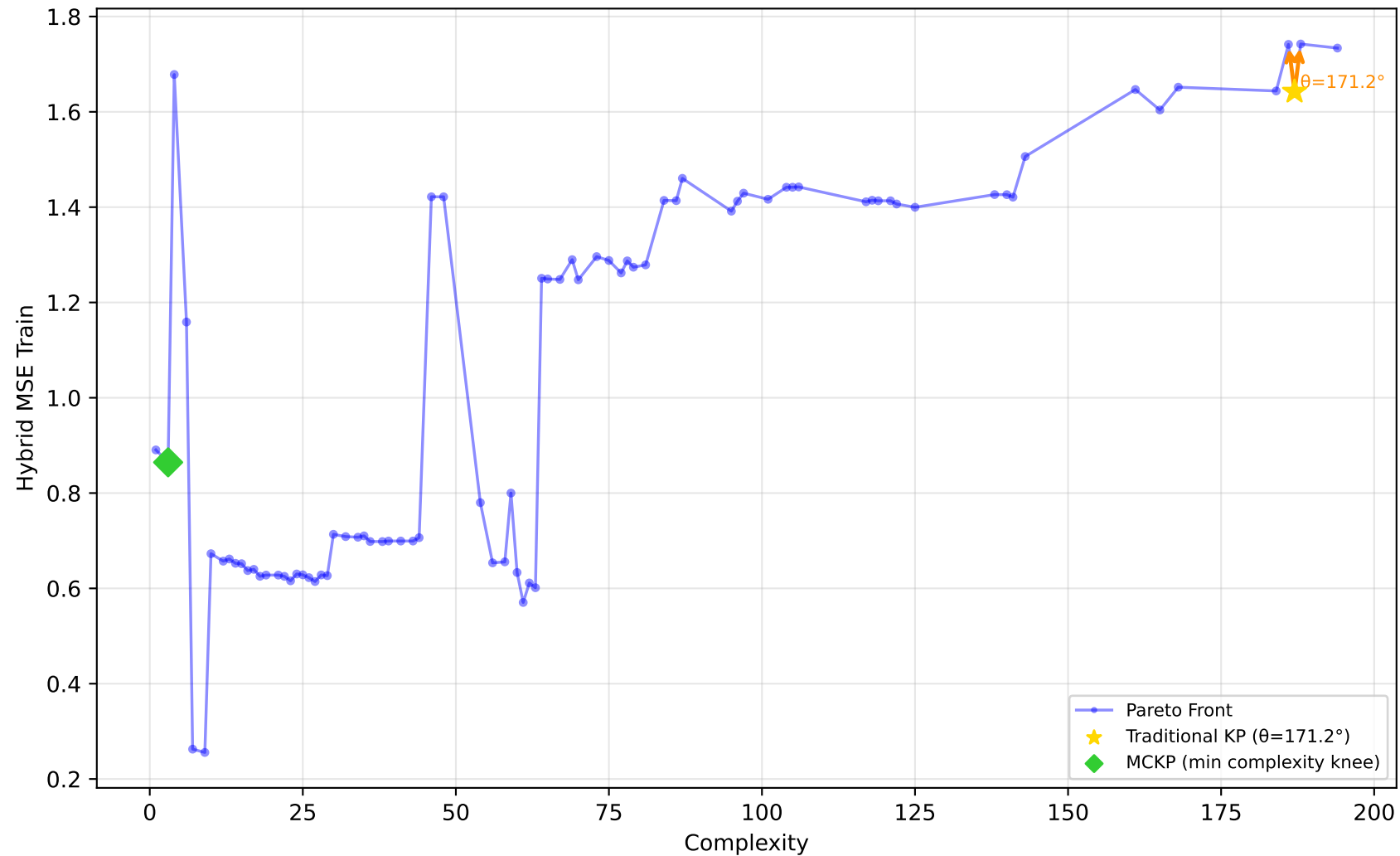
228_elusage - Run 25 - SVP - Hybrid MSE Train \lambda_1=0.60, \bar{\lambda}_2=0.60, \lambda_3=1.00 | Difficulty: 0.87 | Method: hmr
