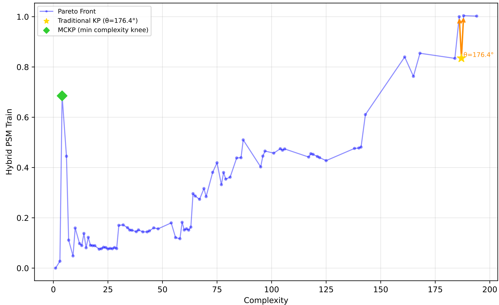
228_elusage - Run 25 - SVP - Hybrid PSM Train \lambda_1=0.00, \bar{\lambda}_2=1.00, \lambda_3=0.00 | Difficulty: 0.87 | Method: hmr
