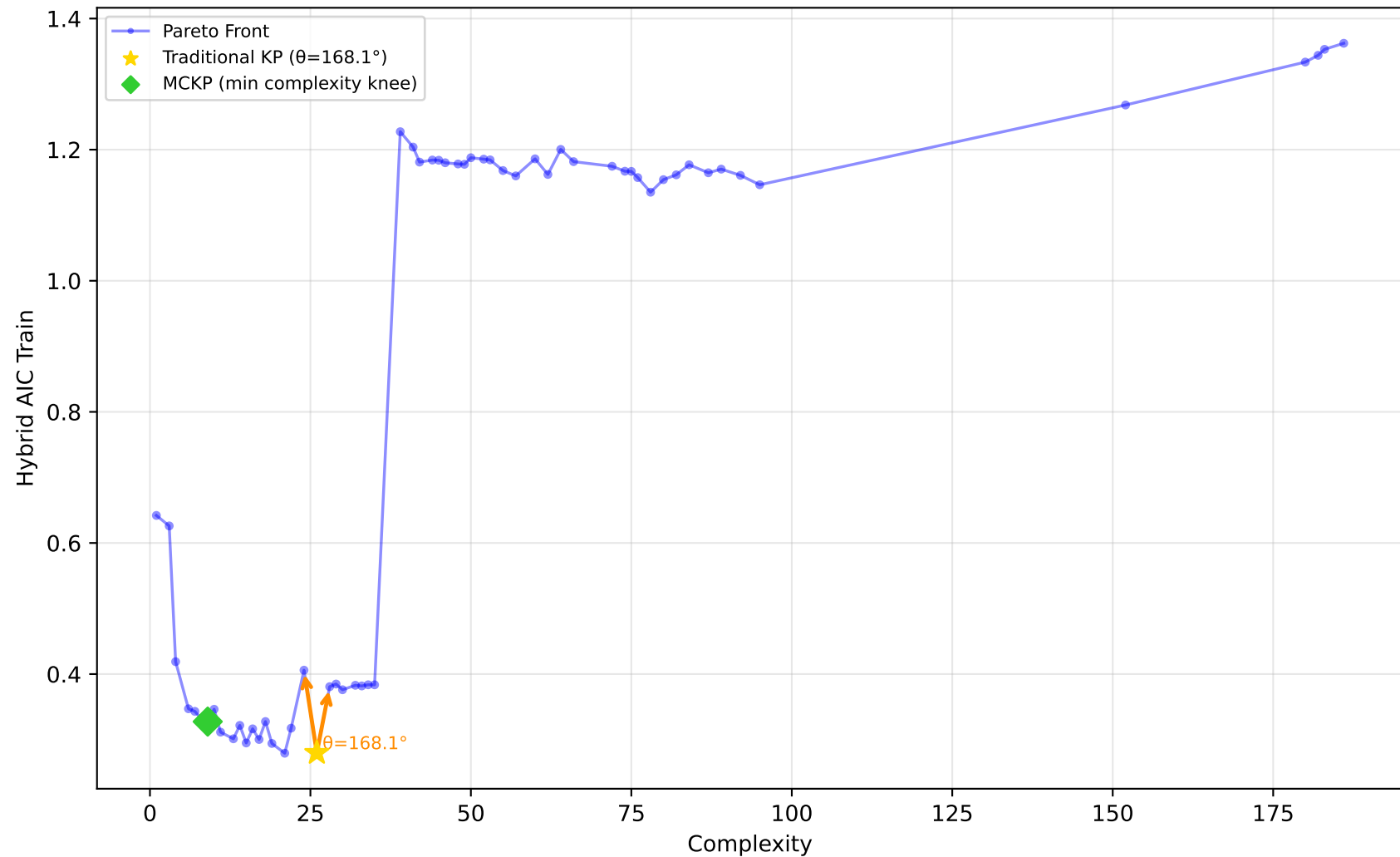
228_elusage - Run 26 - MVP - Hybrid AIC Train \lambda_1=0.00, \lambda_2=0.00, \lambda_3=1.00 | Difficulty: 0.44 | Method: mckp
